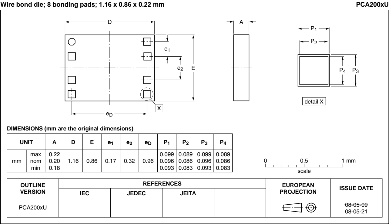
Fig 13. Bare die outline PCA2000U and PCA2001U
