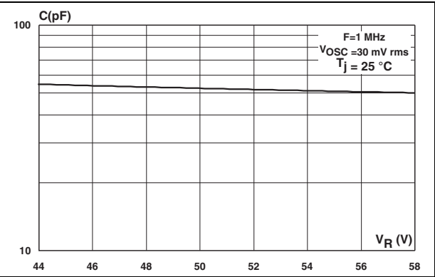
Figure 6. Capacitance versus voltage (typical values)
