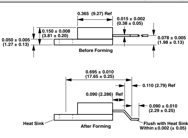
FIGURE 3 - VPR220SZ FORMING DIMENSIONS in inches (millimeters)
