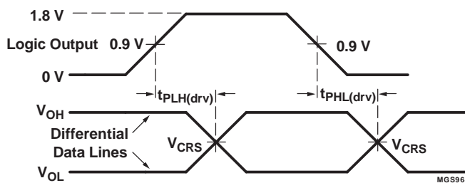
Figure 4. VO/VP, FSE0/VMO to D+, D–
