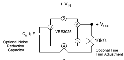
Figure 3 External Connections
