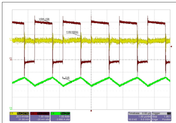
Figure 9. VDDQ output ripple and phase @ AVG current
