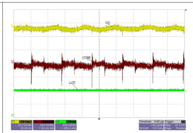
Figure 10. VTT, VTTREF output ripple @ AVG current
