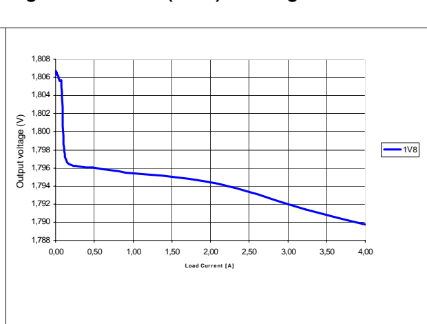
Figure 14. VDDQ (1.8 V) load regulation
