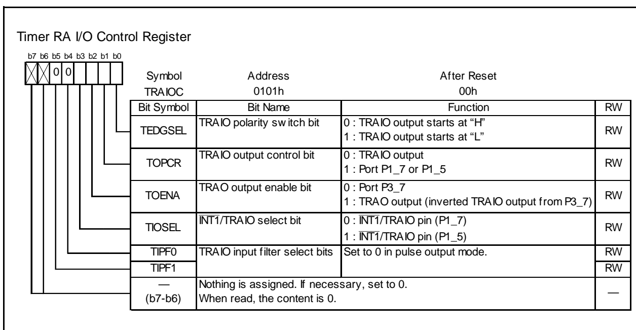
Figure 14.6 TRAI/O Register in Pulse Output Mode
