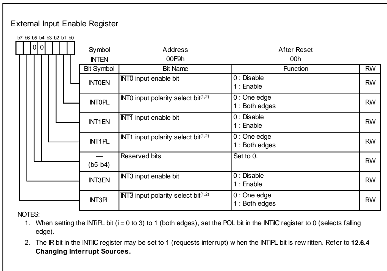
Figure 12.12 \text{INTEN} Register
