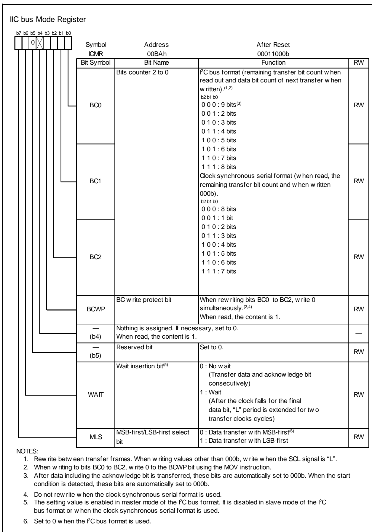
Figure 16.26 ICMR Register
