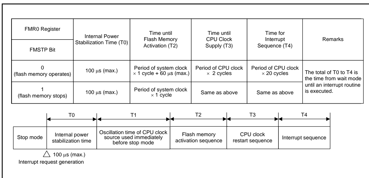
Figure 10.4 Time from Stop Mode to Interrupt Routine Execution
