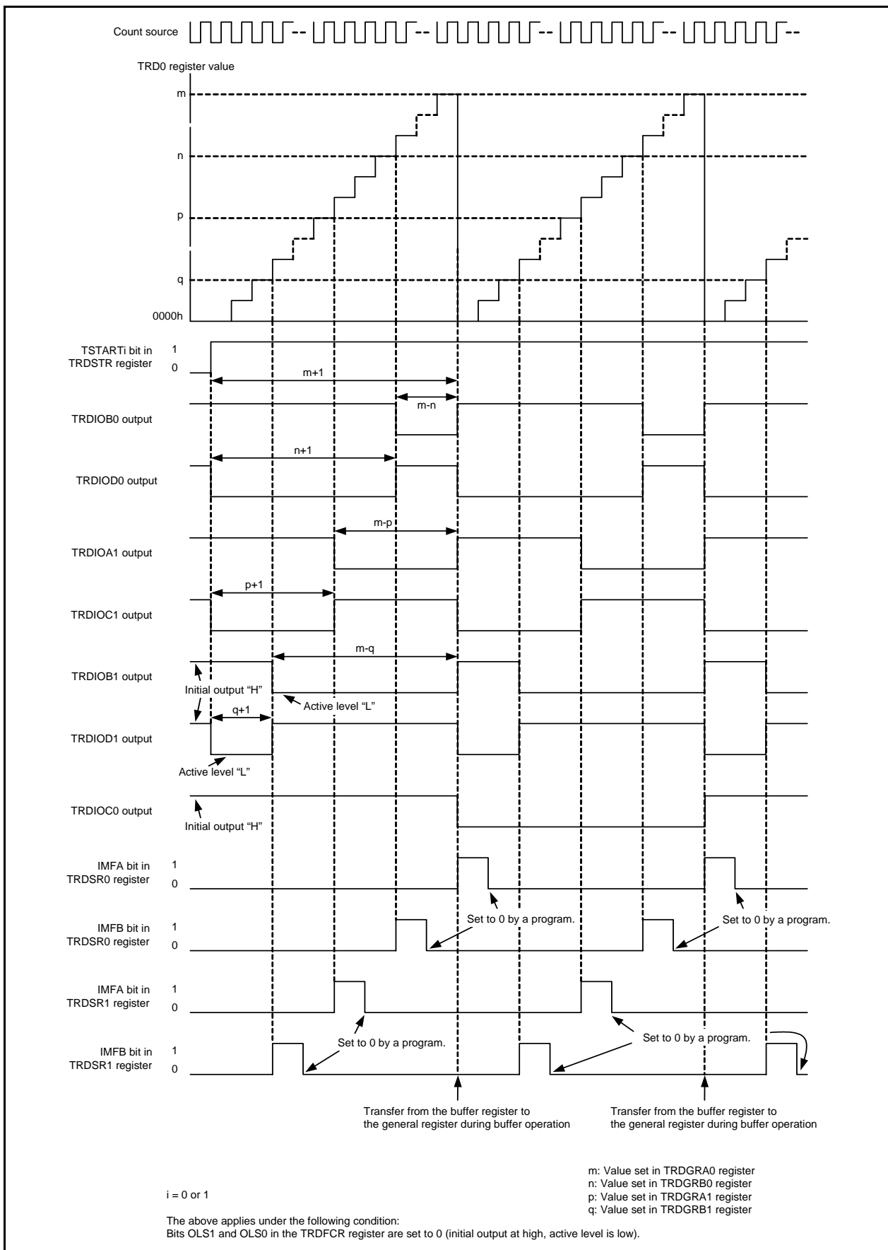
Figure 21.18 Operating Example in Reset Synchronous PWM Mode
