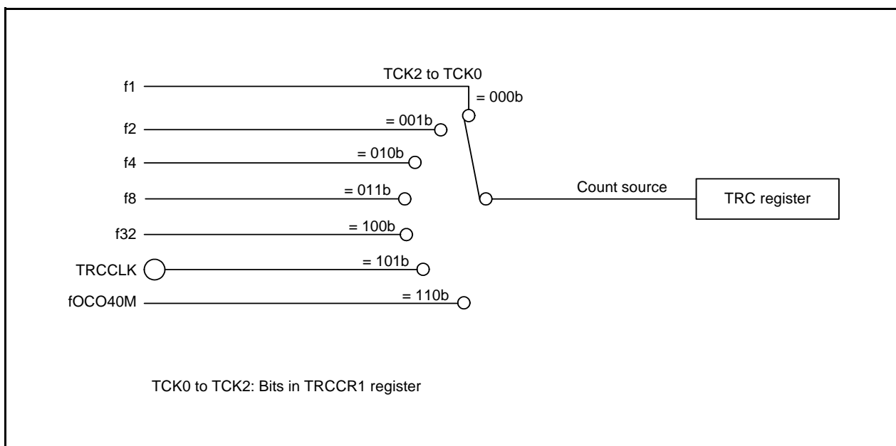
Figure 20.2 Count Source Block Diagram
