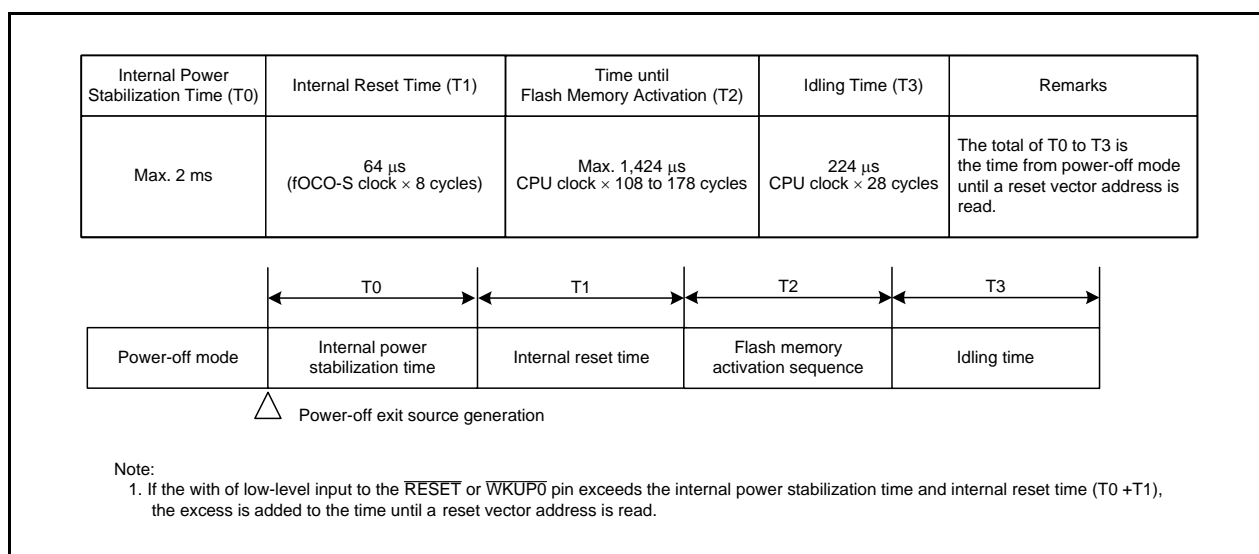
Figure 10.6 Time from Power-Off Mode to Reset Vector Address Read Execution
