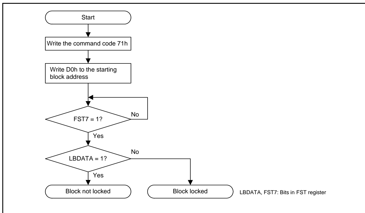
Figure 35.13 Read Lock Bit Status Flowchart
