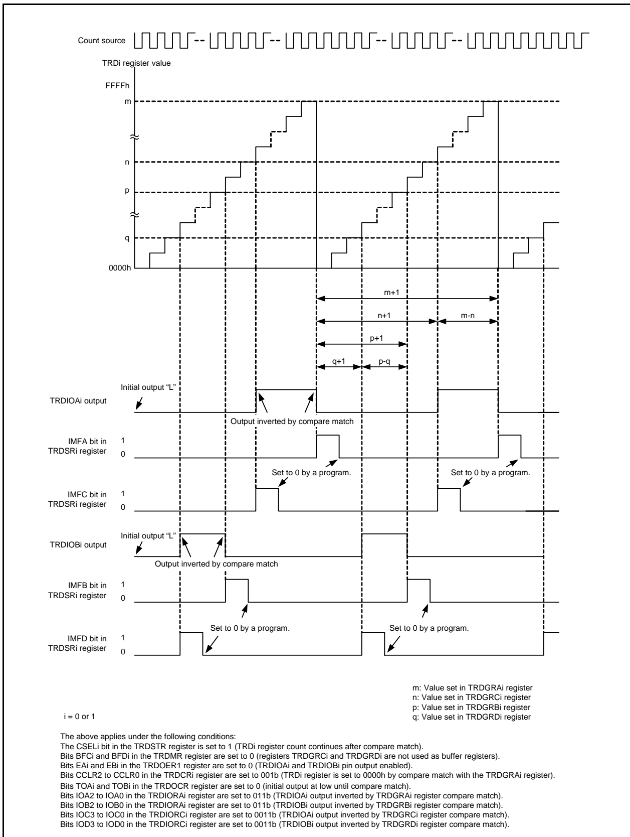
Figure 21.13 Operating Example When TRDGRCi Register is Used for Output Control of TRDIOAi Pin and TRDGRDi Register is Used for Output Control of TRDIOBi Pin
