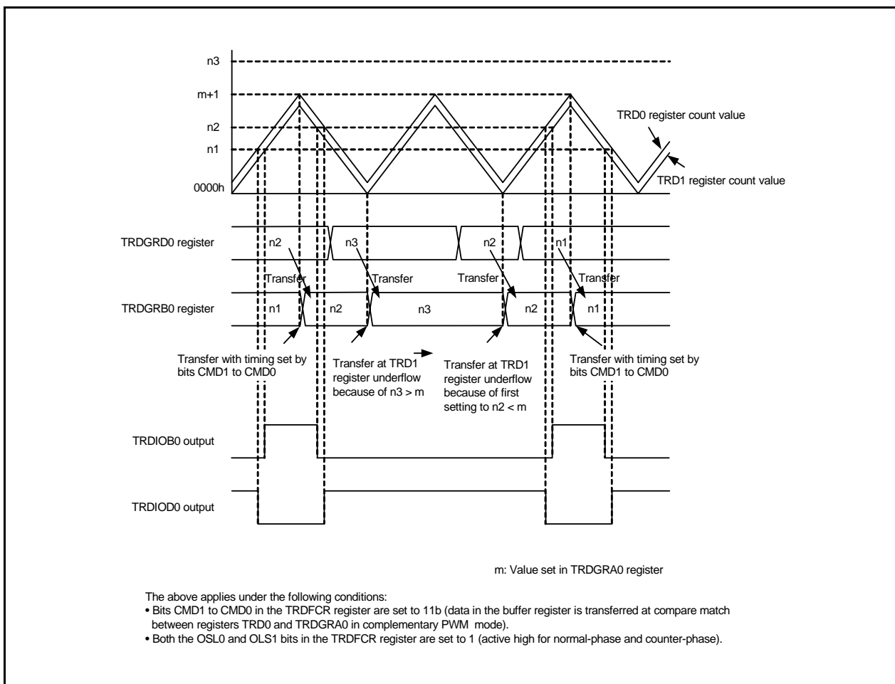
Figure 21.27 Operation when Buffer Register Value \geq TRDGRA0 Register Value in Complementary PWM Mode
