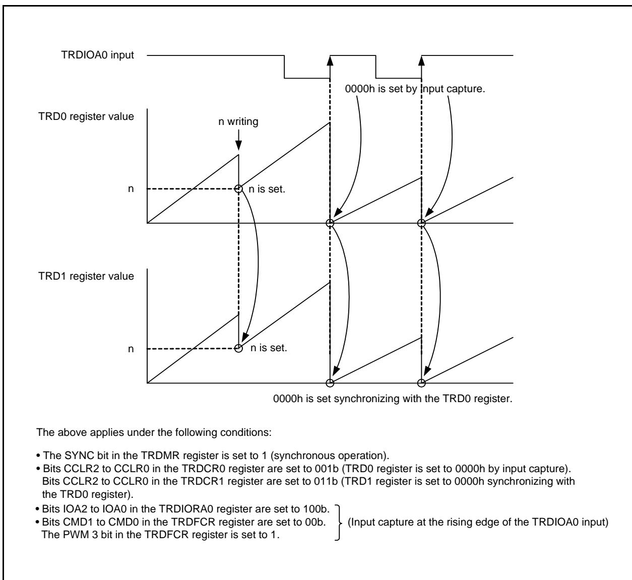
Figure 21.5 Synchronous Operation
