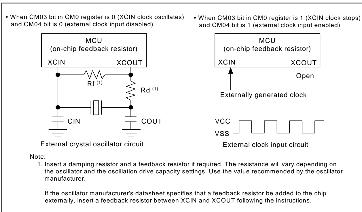
Figure 9.4 Examples of XCIN Clock Connection Circuits
