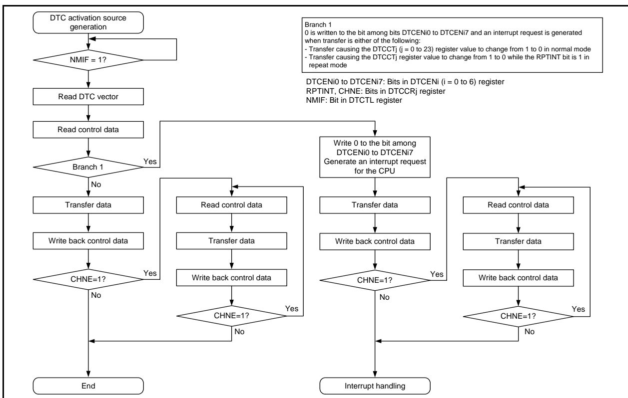
Figure 16.3 DTC Internal Operation Flowchart When DTC Activation Source is not SSU/I²C bus, Timer RC, Timer RD, or Flash Memory Interrupt Source
