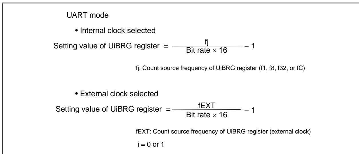
Figure 24.8 Formula for Calculating Setting Value of UiBRG Register (i = 0 or 1)
