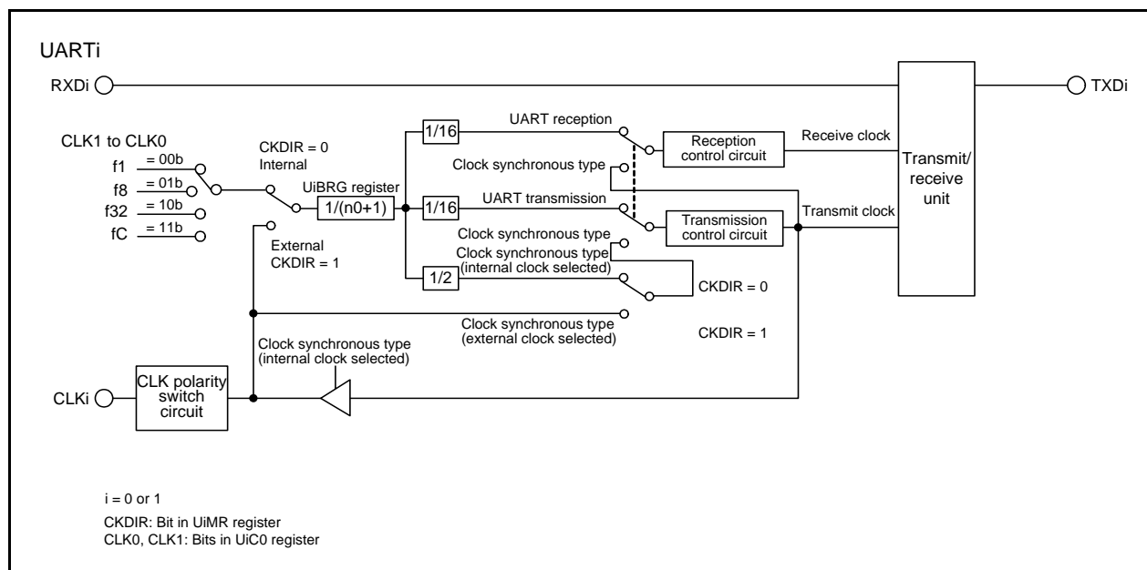
Figure 24.1 Block Diagram of UARTi (i = 0 or 1)
