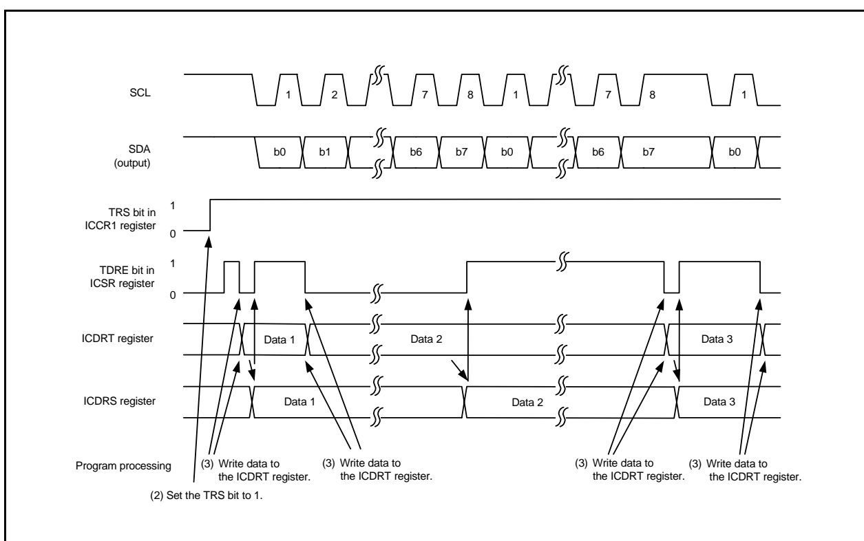
Figure 28.13 Operating Timing in Transmit Mode (Clock Synchronous Serial Mode)
