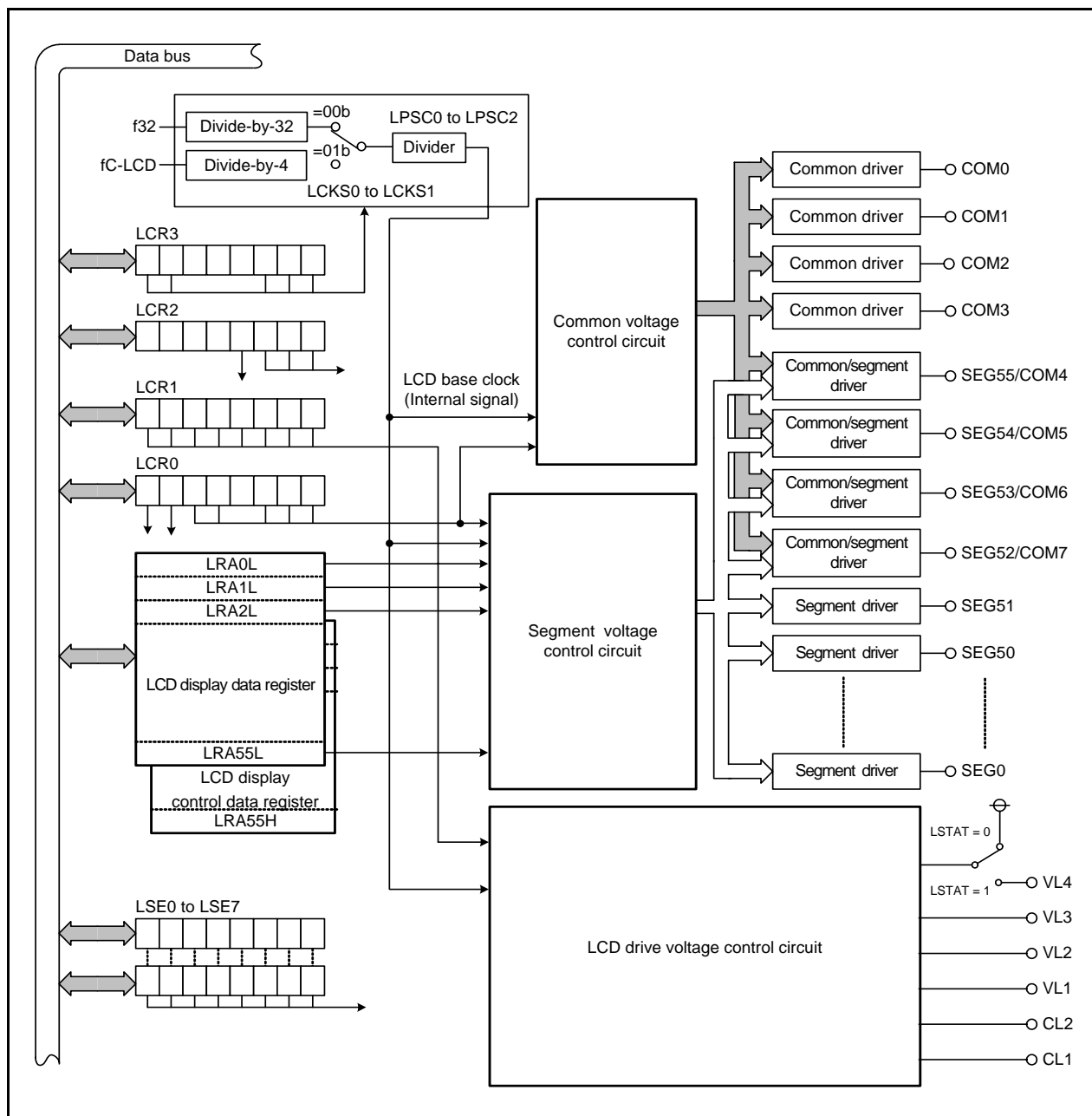
Figure 34.1 Block Diagram of LCD Drive Control Circuit
