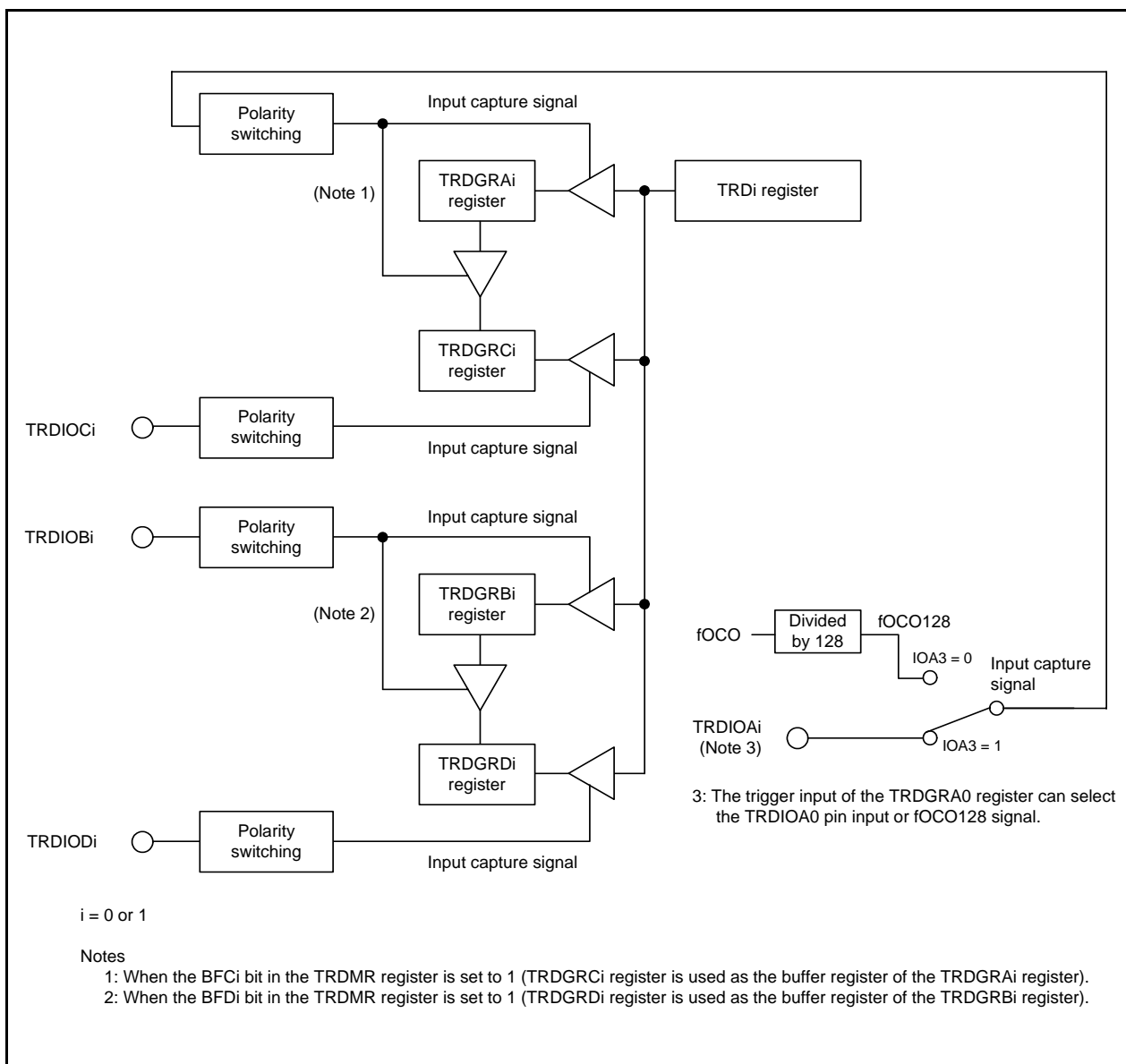
Figure 21.7 Block Diagram of Input Capture Function
