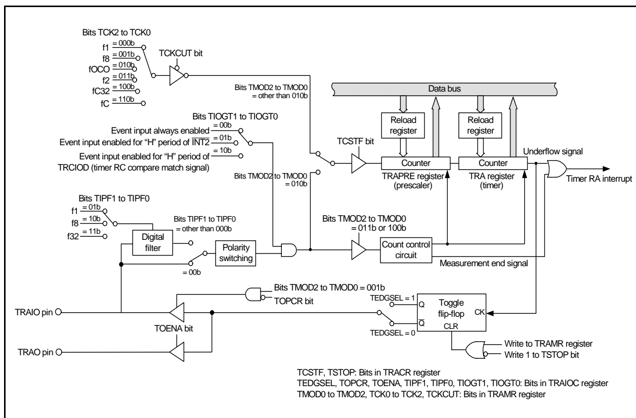
Figure 18.1 Timer RA Block Diagram
