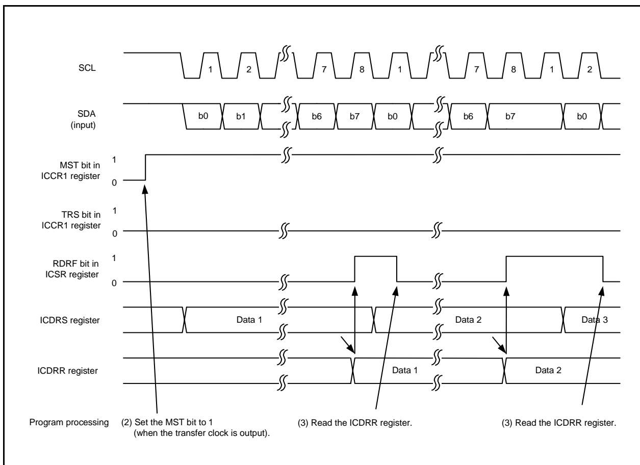
Figure 28.14 Operating Timing in Receive Mode (Clock Synchronous Serial Mode)
