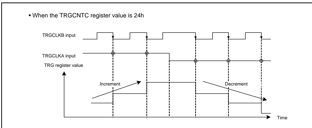
Figure 23.18 Operating Example in Phase Counting Mode 2
