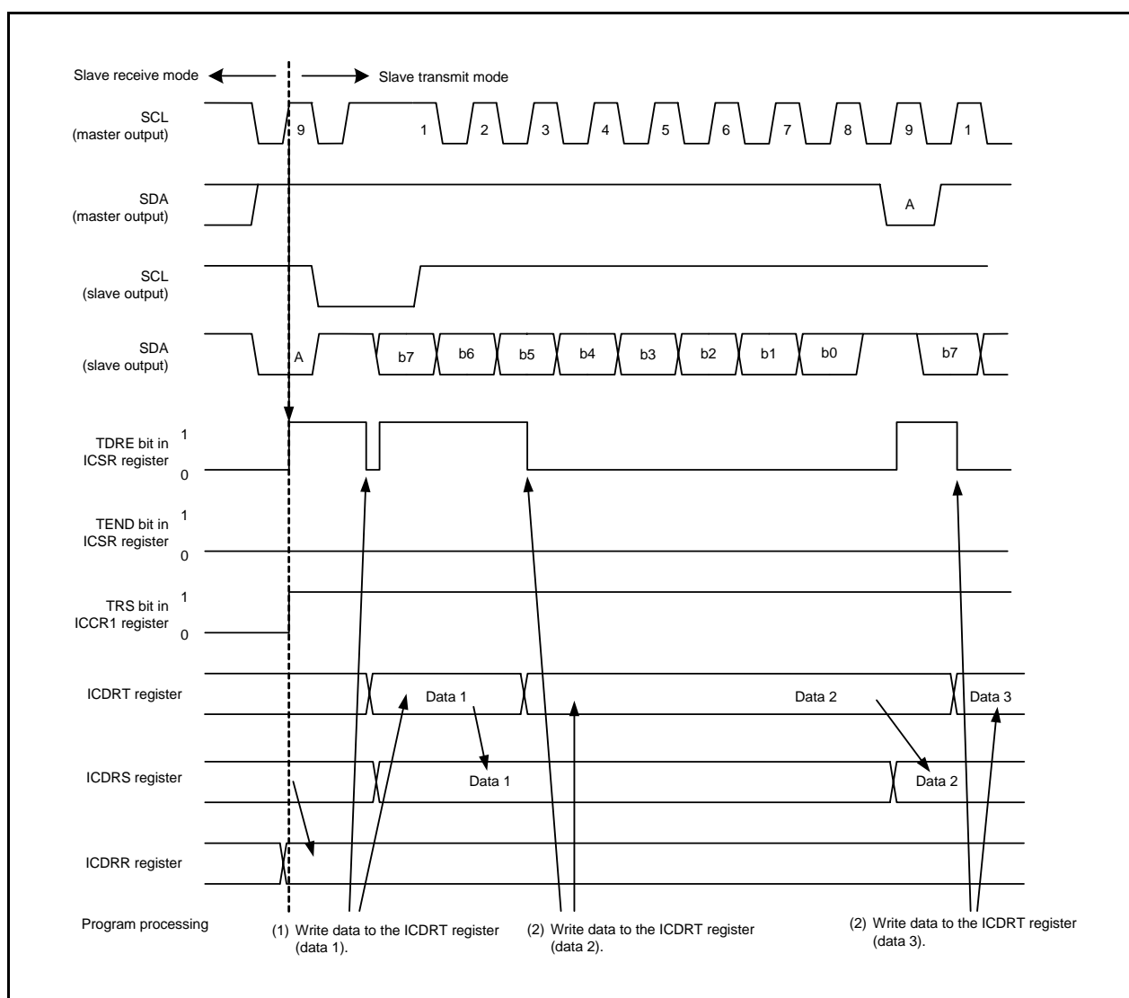
Figure 28.8 Operating Timing in Slave Transmit Mode (I 2 C bus Interface Mode) (1)
