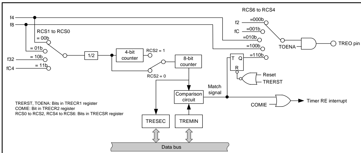
Figure 22.4 Block Diagram of Output Compare Mode
