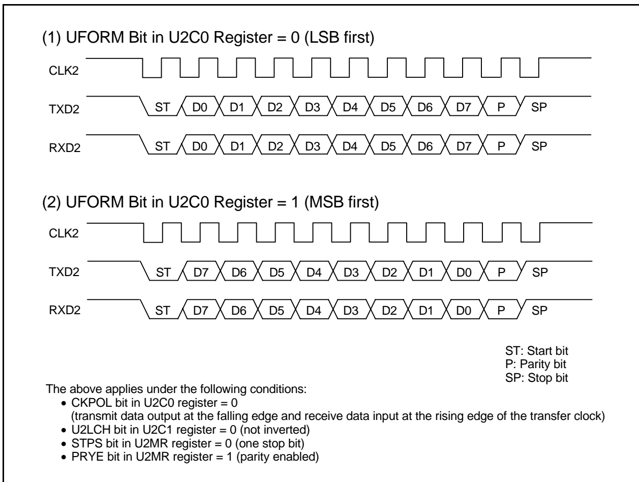
Figure 25.9 Transfer Format
