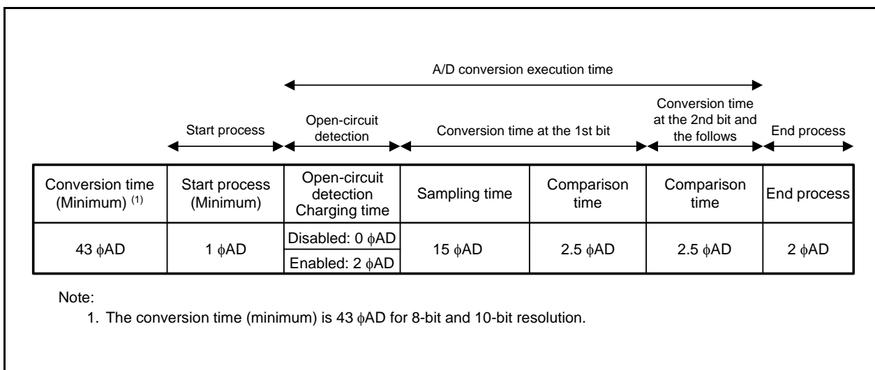
Figure 30.3 A/D Conversion Cycles ( \phi_{AD} = f_{AD} )
