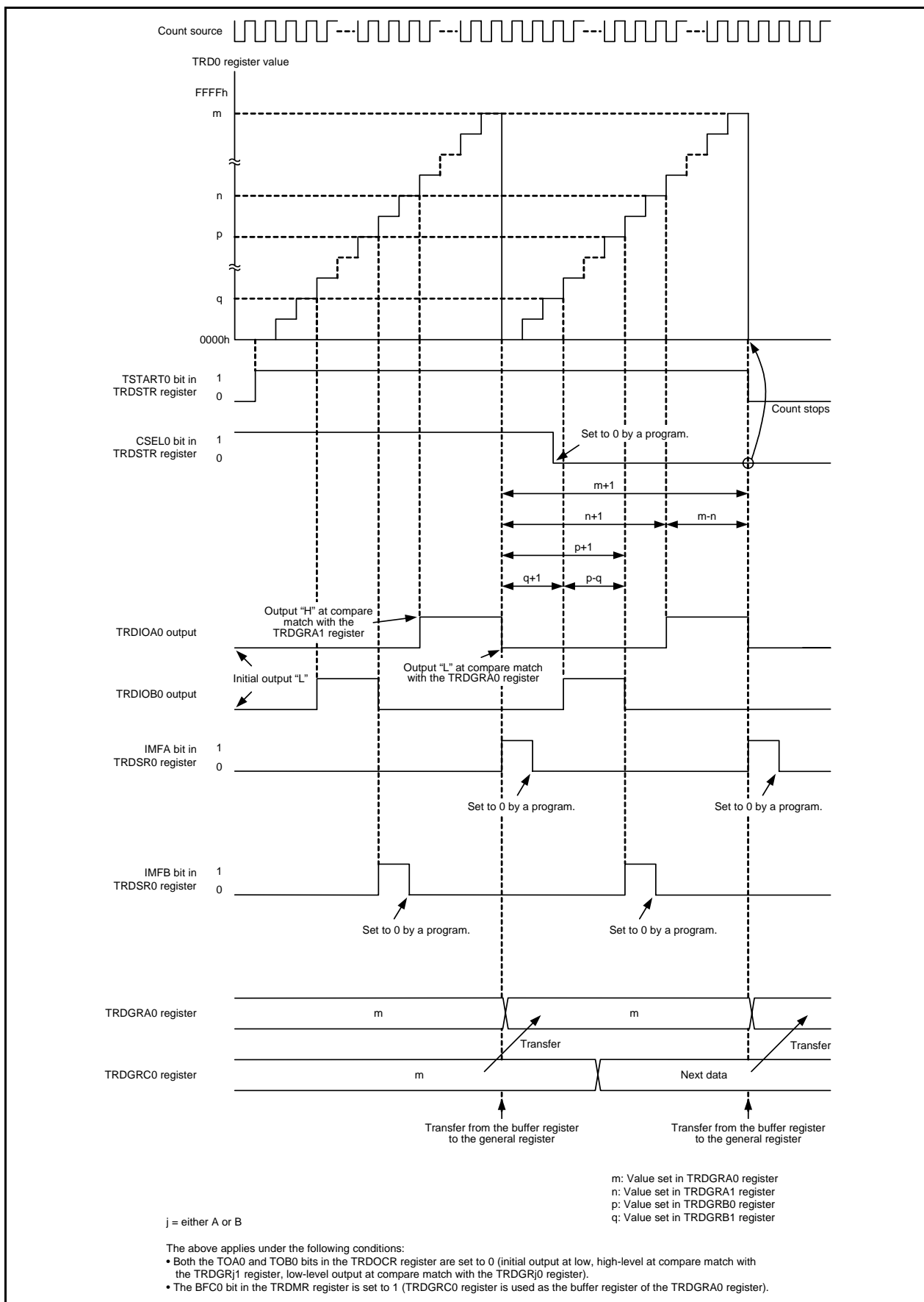
Figure 21.23 Operating Example in PWM3 Mode
