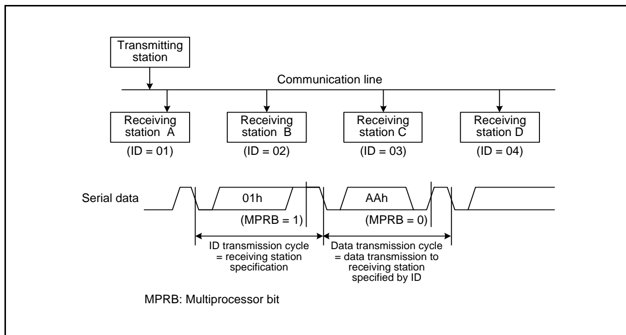
Figure 25.17 Multiprocessor Communication Example Using Multiprocessor Format (Data AAh Transmission to Receiving Station A)
