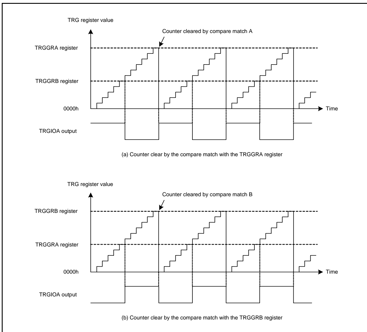
Figure 23.14 Operating Example in PWM Mode (1)
