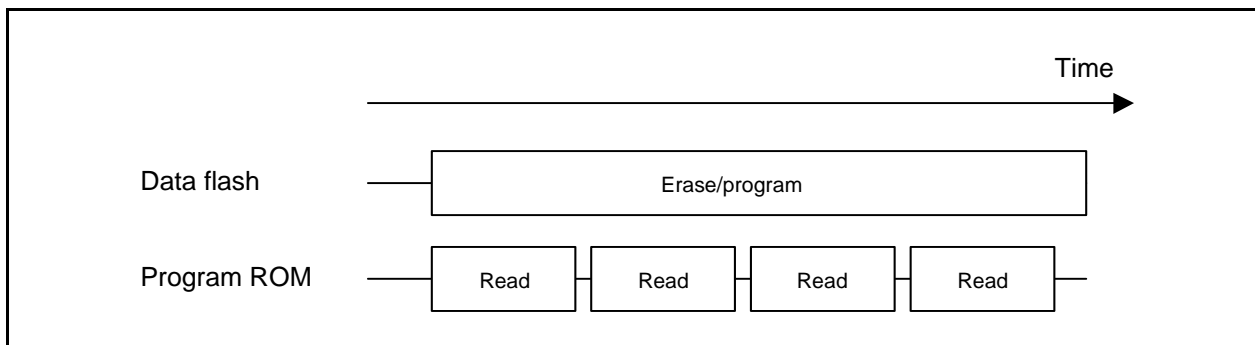
Figure 35.5 BGO Function
