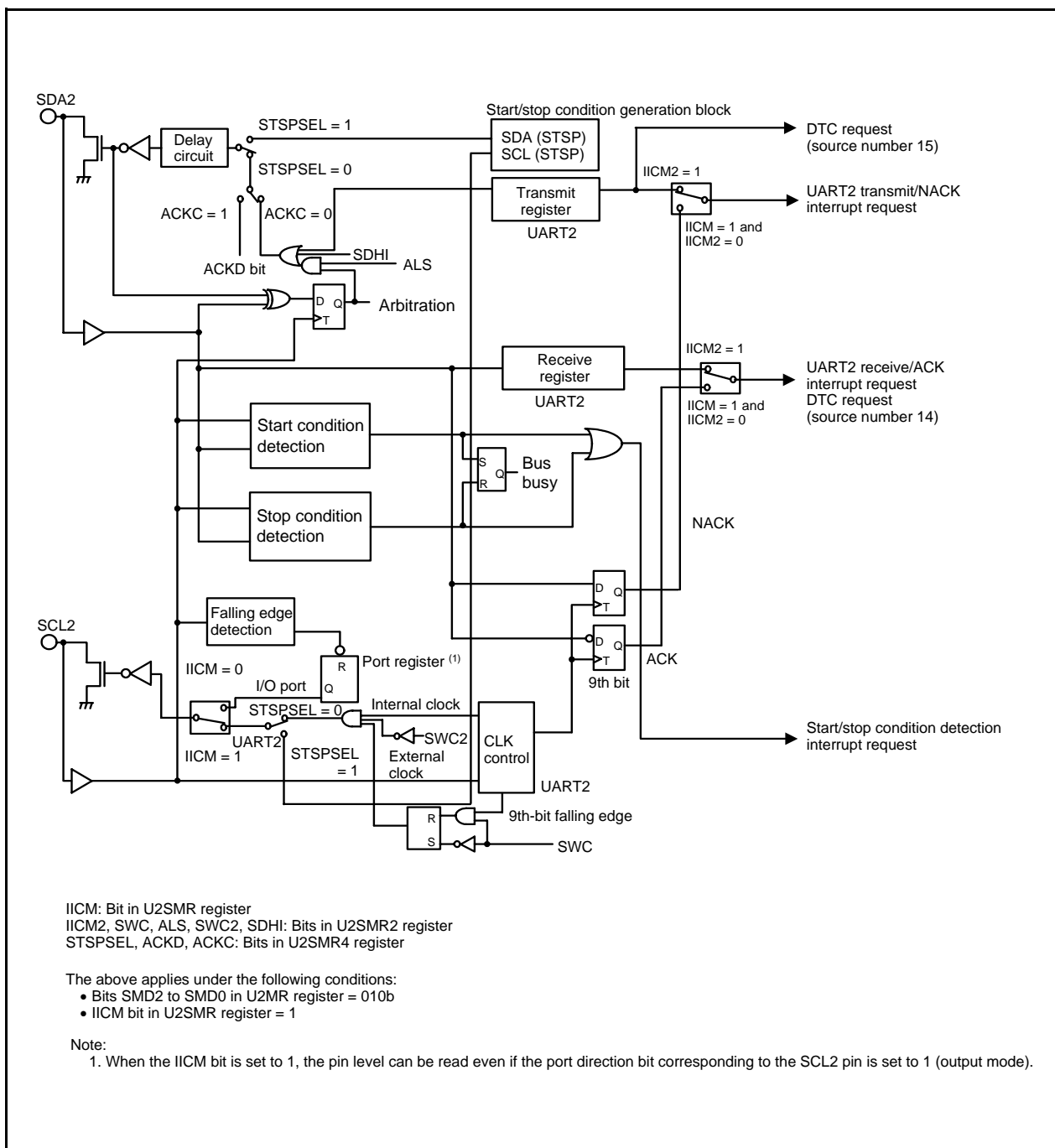
Figure 25.13 Block Diagram of I²C Mode
