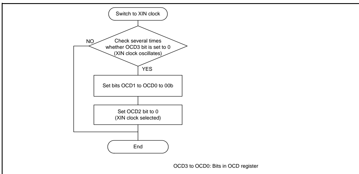
Figure 9.5 Procedure for Switching Low-Speed On-Chip Oscillator to XIN Clock
