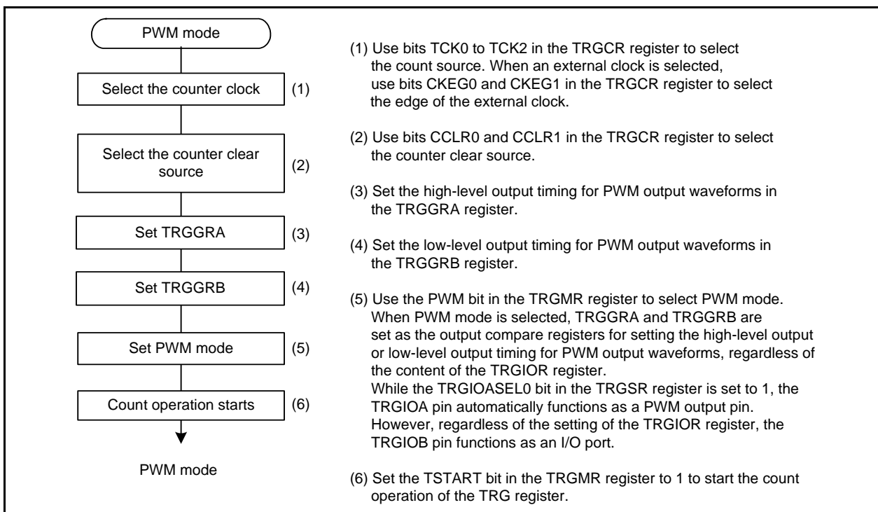
Figure 23.13 Procedure Example for Setting PWM Mode
