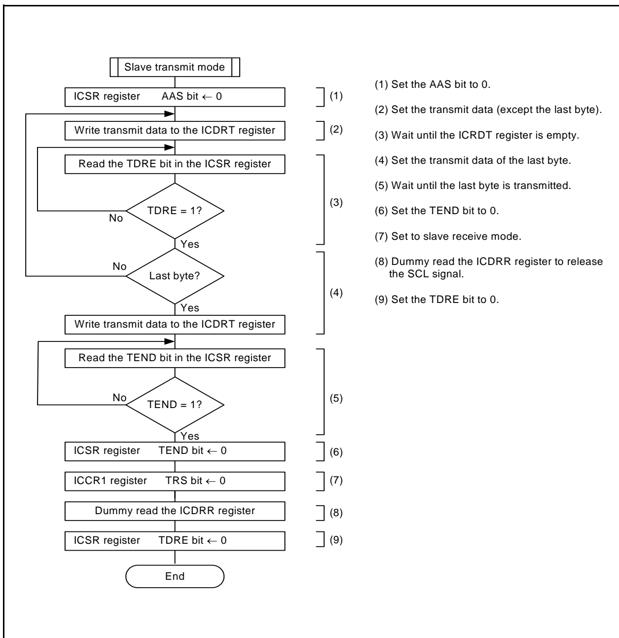
Figure 28.17 Register Setting Example in Slave Transmit Mode (I 2 C bus Interface Mode)
