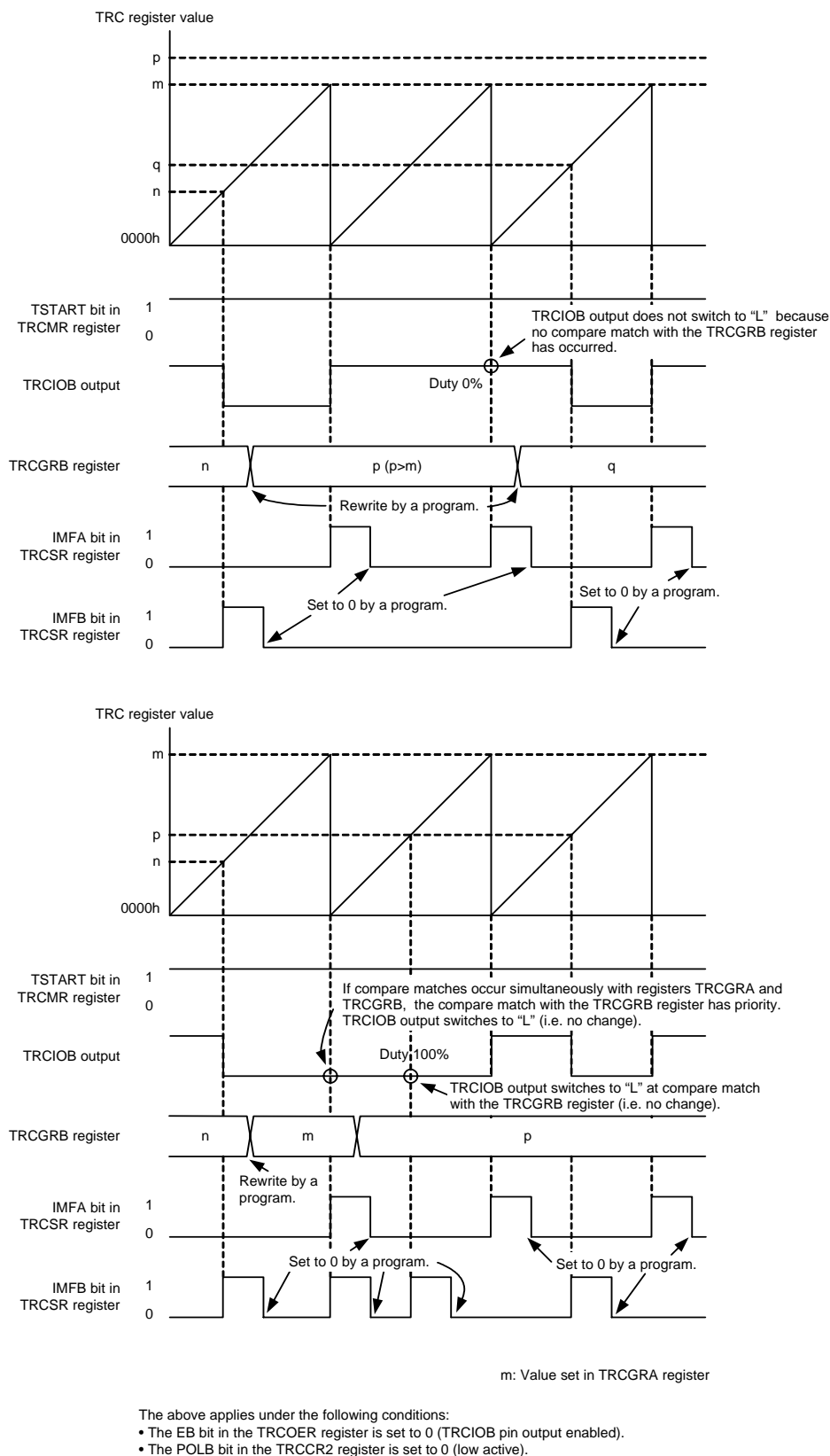
Figure 20.15 Operating Example in PWM Mode (Duty 0% and Duty 100%)
