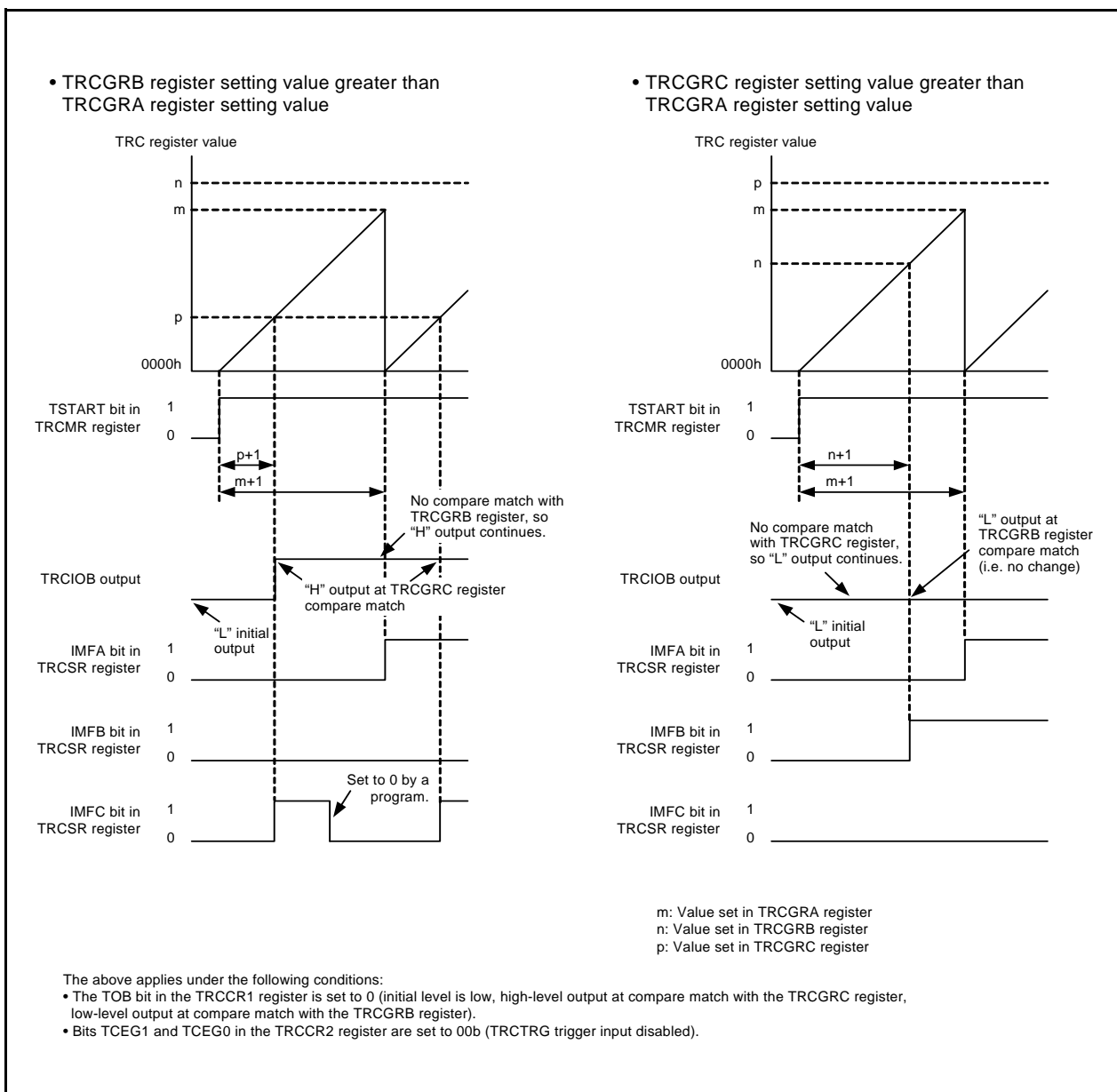
Figure 20.19 Operating Example in PWM2 Mode (Duty 0% and Duty 100%)
