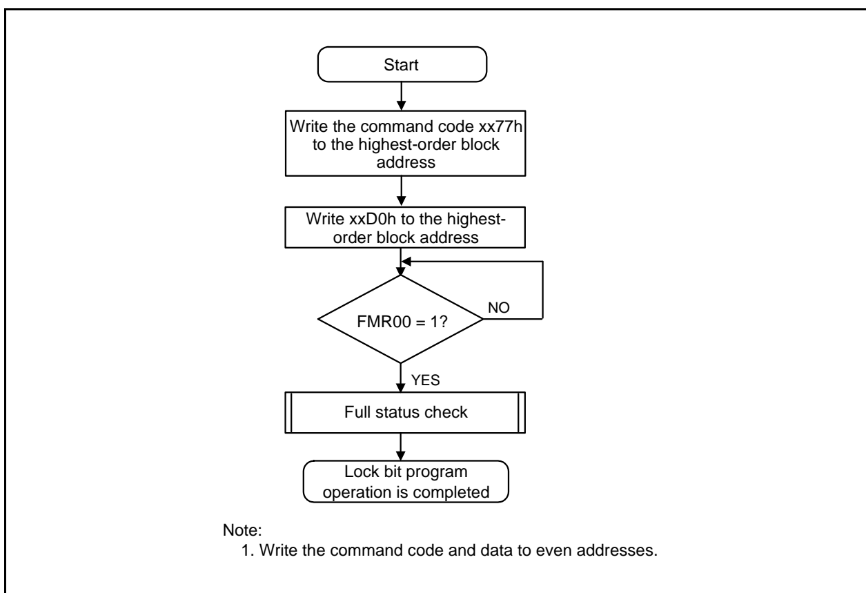
Figure 30.5 Lock Bit Program Command (Suspend Function Disabled)
