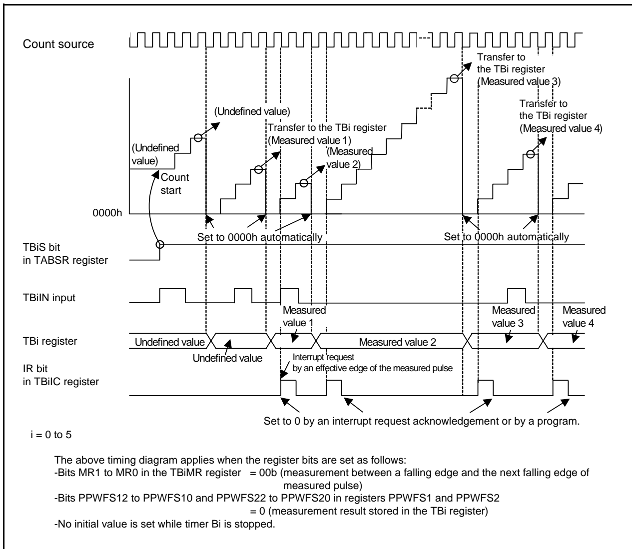
Figure 18.6 Operation Example in Pulse Period Measurement Mode
