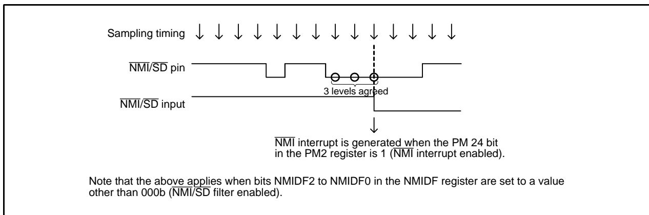
Figure 13.11 \overline{\text{NMI}}/\overline{\text{SD}} Digital Filter
