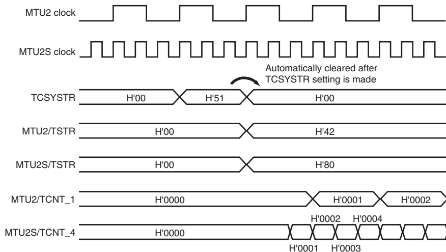
Figure 11.84 (3) Example of Synchronous Counter Start Operation (MTU2-to-MTU2S Clock Frequency Ratio = 1:3)
