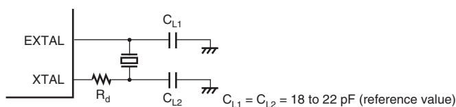
Figure 4.2 Example of Crystal Resonator Connection
