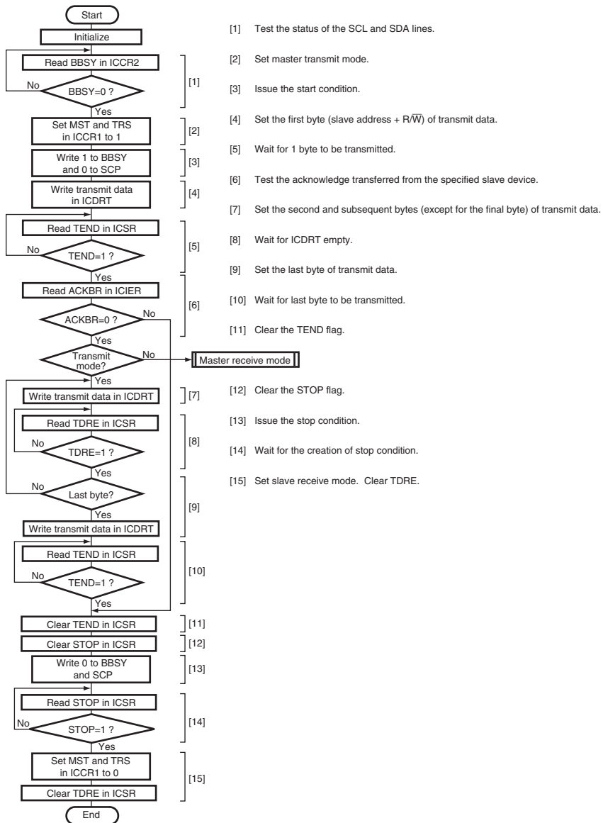
Figure 19.18 Sample Flowchart for Master Transmit Mode
