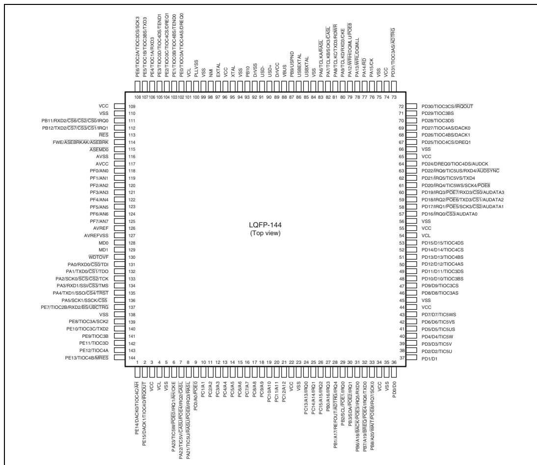
Figure 1.3 SH7285 Pin Assignment
