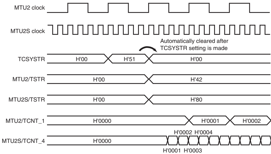
Figure 11.84 (4) Example of Synchronous Counter Start Operation (MTU2-to-MTU2S Clock Frequency Ratio = 1:4)
