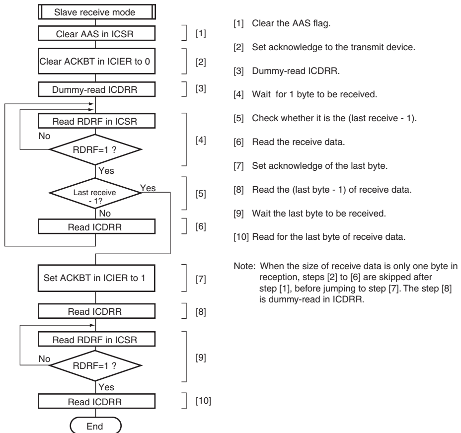
Figure 19.21 Sample Flowchart for Slave Receive Mode
