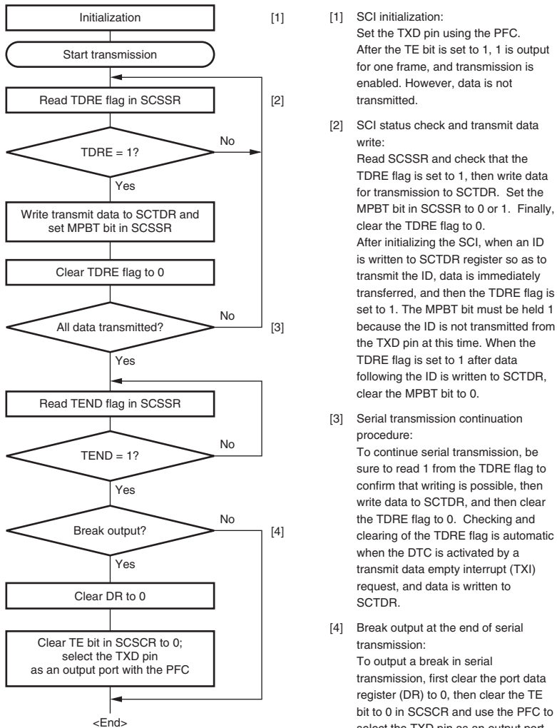
Figure 16.16 Sample Multiprocessor Serial Transmission Flowchart
