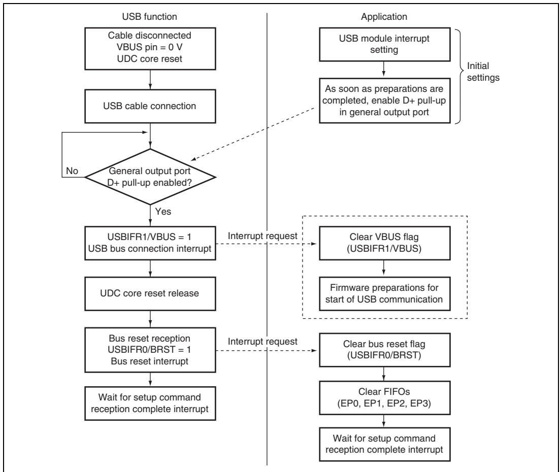
Figure 25.2 Cable Connection Operation
