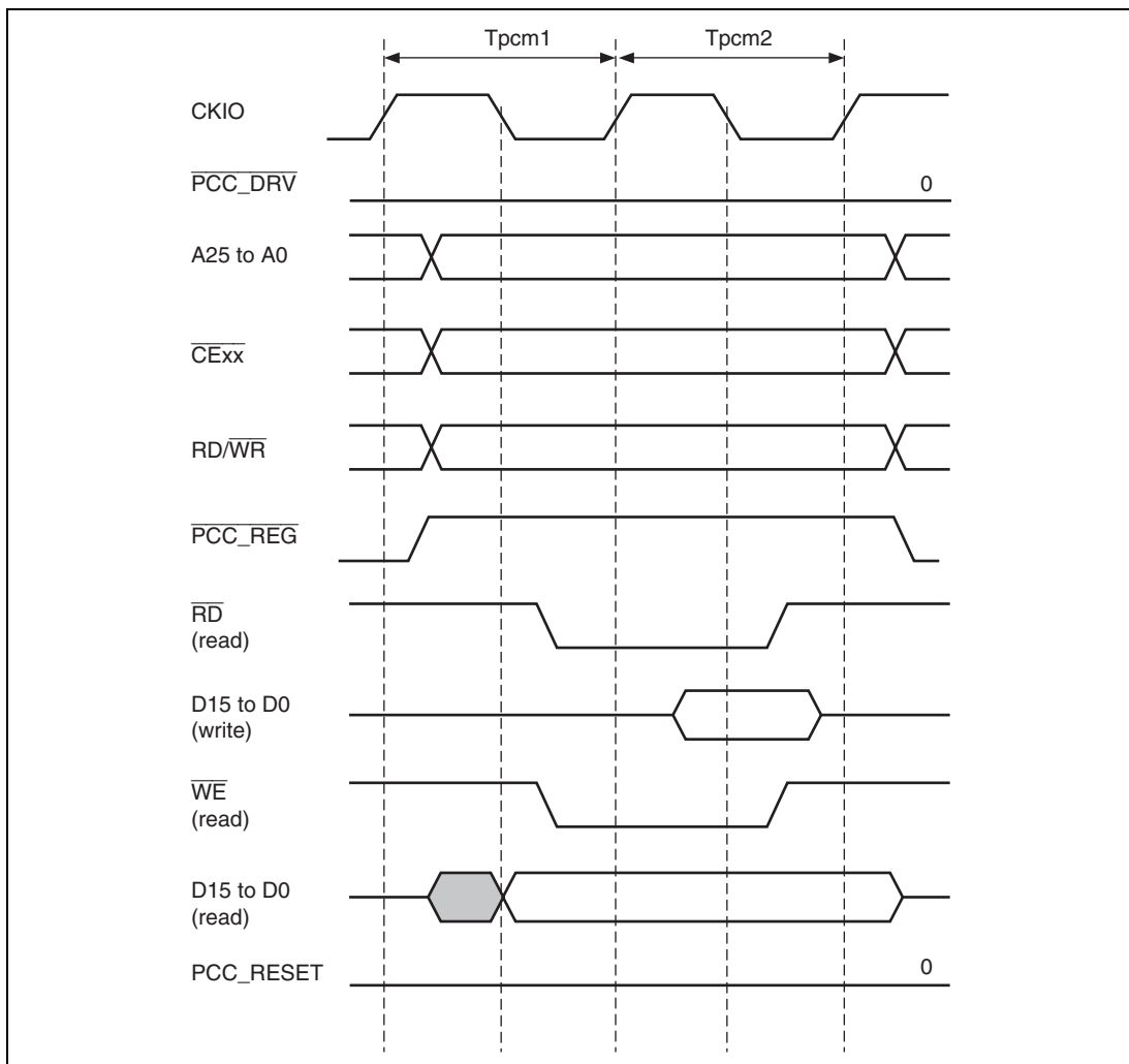
Figure 29.5 PCMCIA Memory Card Interface Basic Timing
