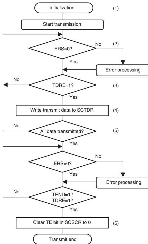
Figure 30.5 Example of Transmit Processing
