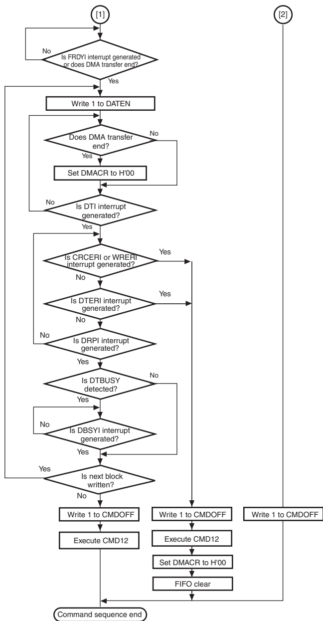
Figure 31.29 Operational Flowchart for Write Sequence (Open-ended Multiblock Transfer) (2)
