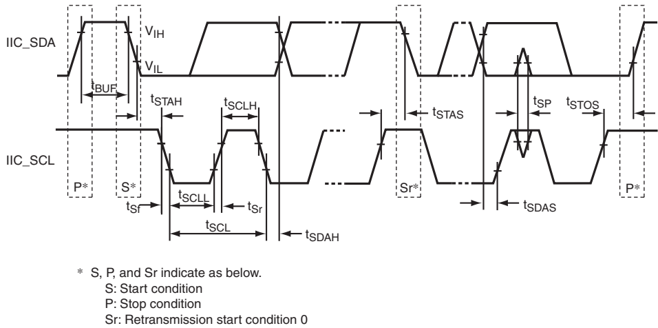
Figure 38.52 I 2 C Bus Interface Input/Output Timing
