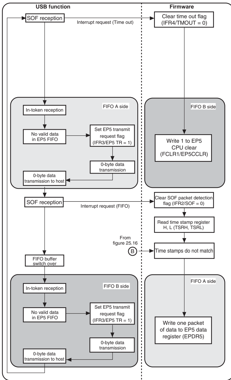
Figure 25.17 EP5 Isochronous-In Transfer Operation (SOF in Broken)
