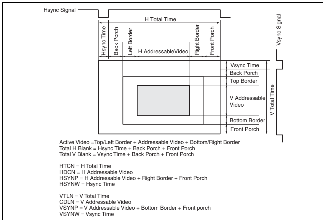
Figure 26.2 Valid Display and the Retrace Period
