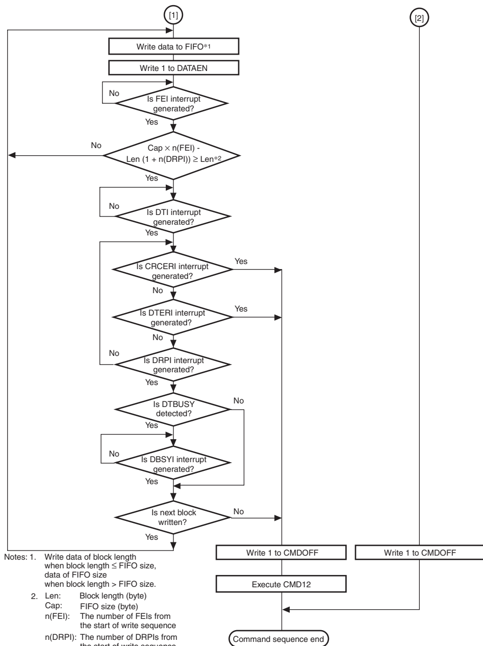
Figure 31.20 Operational Flowchart for Commands with Write Data (Open-ended Multiblock Transfer) (2)
