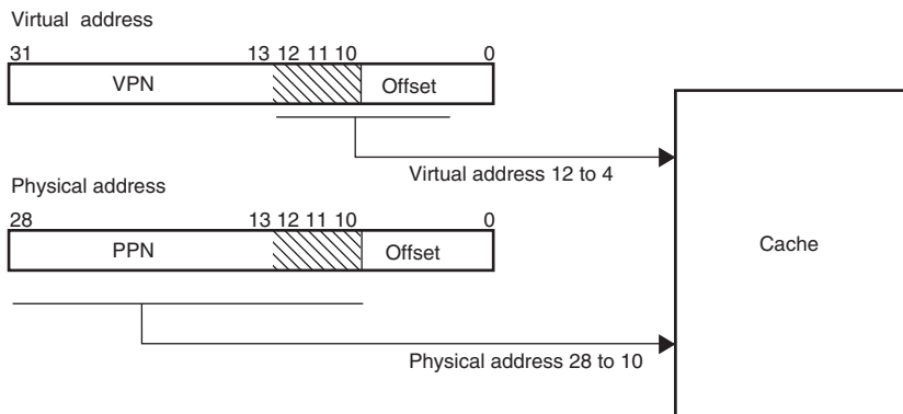
Figure 4.12 Synonym Problem (32-kbyte Cache)
