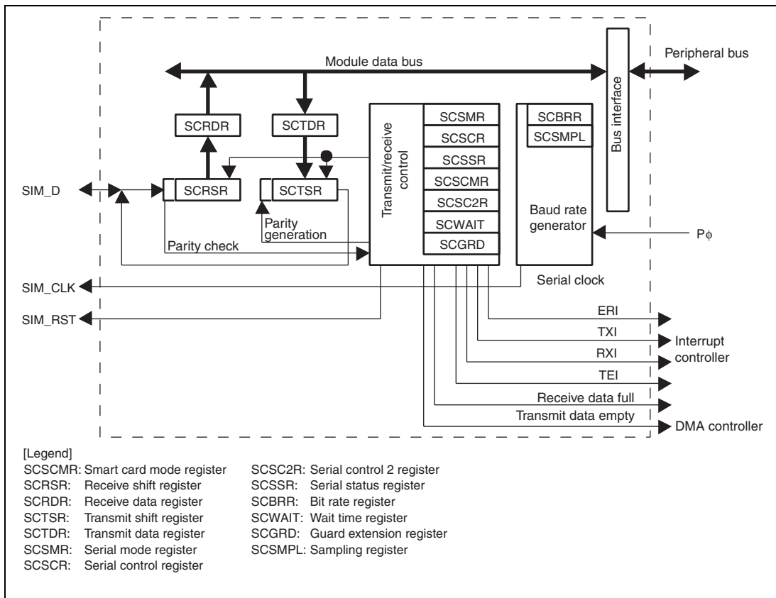
Figure 30.1 Smart Card Interface
