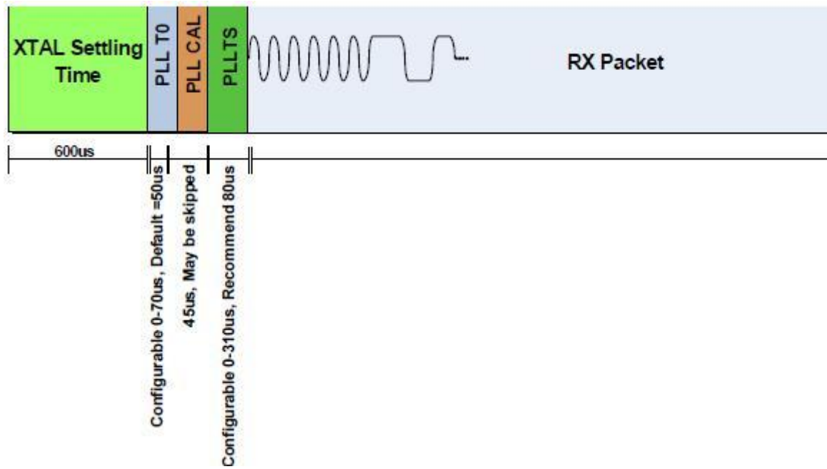
Figure 8. RX Timing
