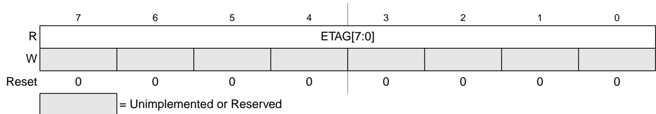
Figure 10-19. EEE Tag Counter Low Register (ETAGLO)
