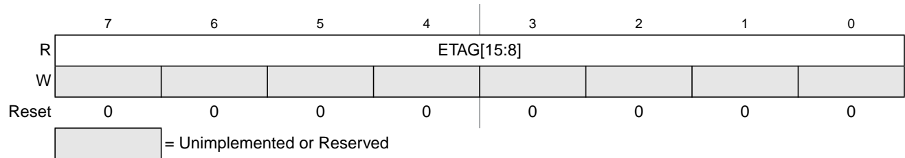
Figure 10-18. EEE Tag Counter High Register (ETAGHI)
