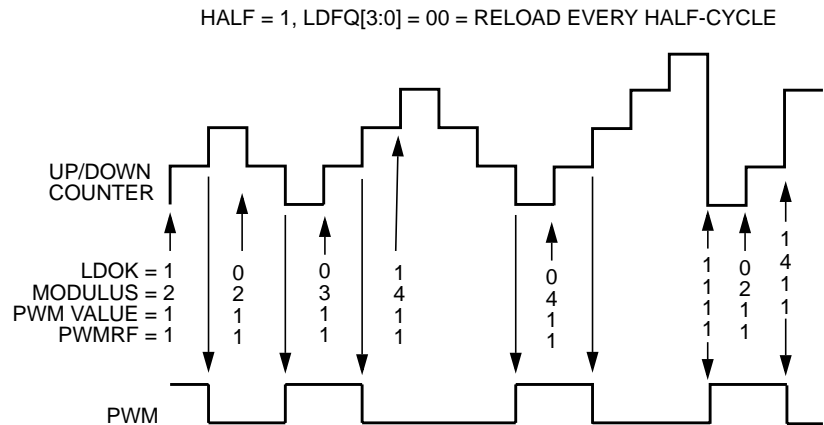
Figure 20-71. Half-Cycle Center-Aligned Modulus Loading
