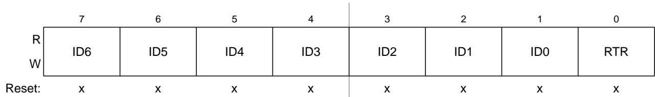
Figure 21-28. Identifier Register 3 (IDR3) — Extended Identifier Mapping
