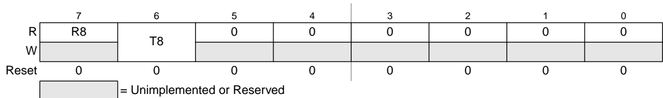
Figure 23-12. SCI Data Registers (SCIDRH)
