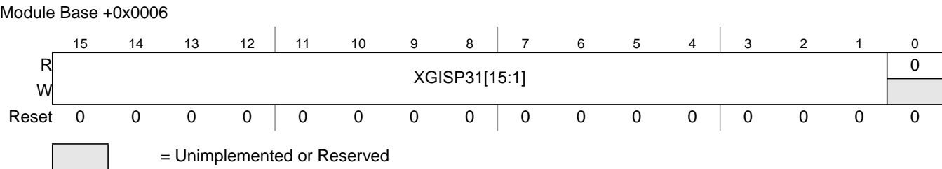
Figure 14-8. XGATE Initial Stack Pointer for Interrupt Priorities 3 to 1 (XGISP31)
