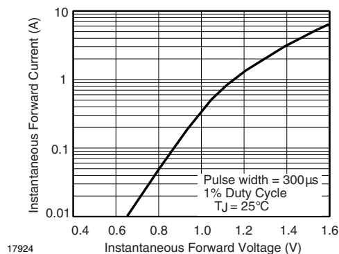
Fig. 4 - Typical Instantaneous Forward Characteristics for SML4763
