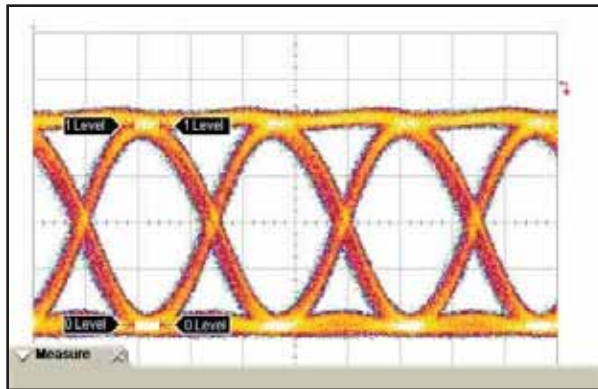
Eye Diagrams
