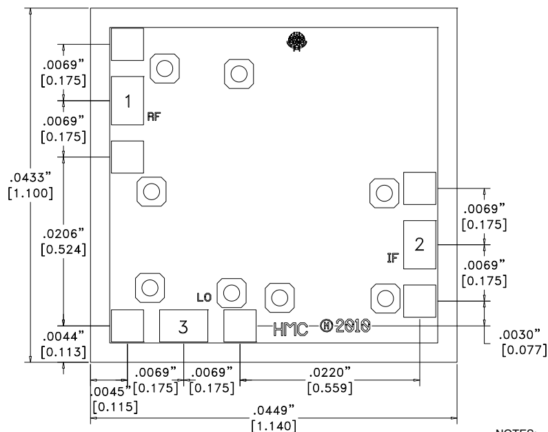
Outline Drawing
