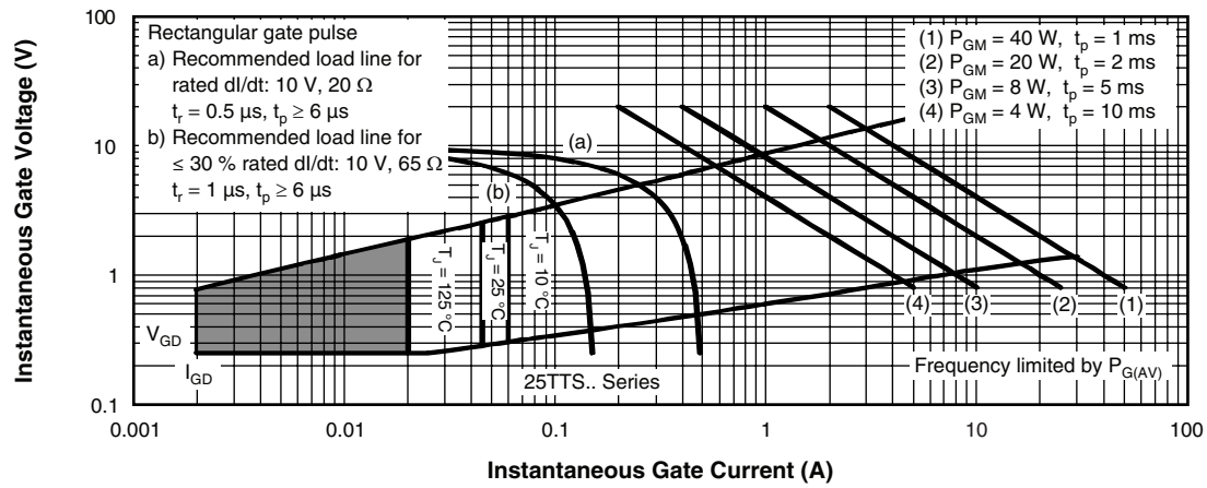
Fig. 8 - Gate Characteristics
