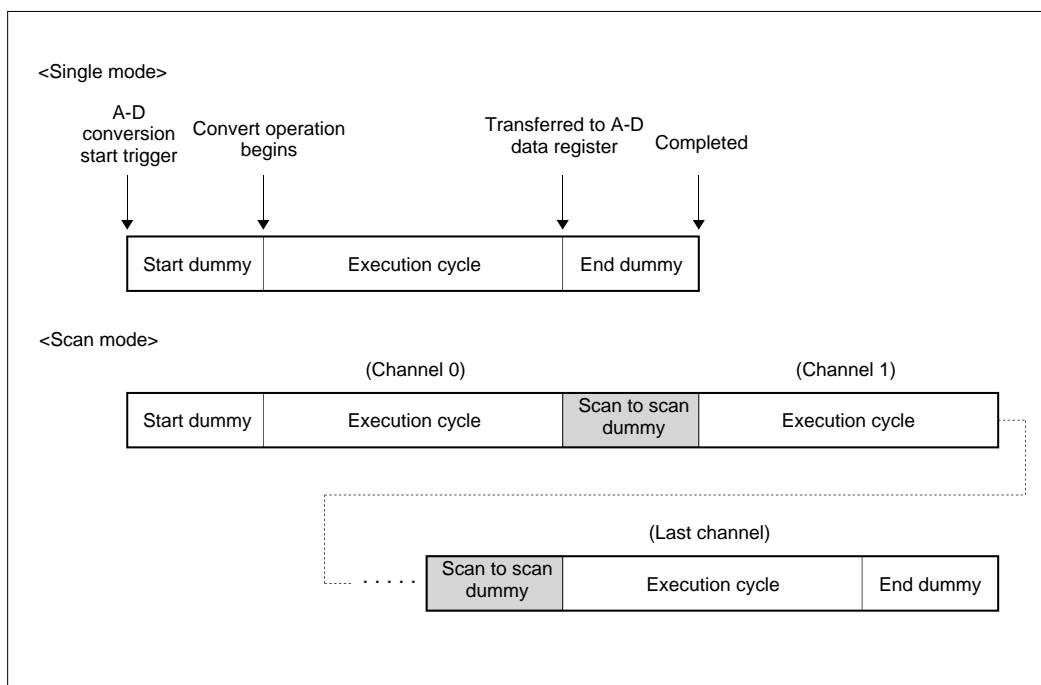
Figure 11.3.3 Conceptual Diagram of A-D Conversion Time
