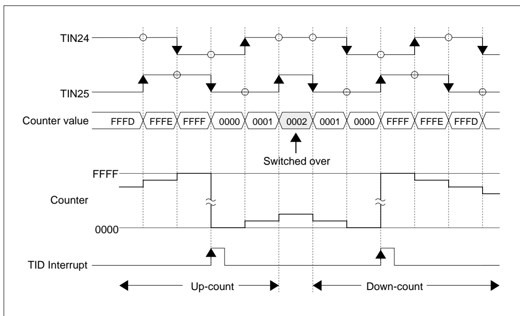
Figure 10.7.8 Up/Down Count Operation (Interrupt Timing)
