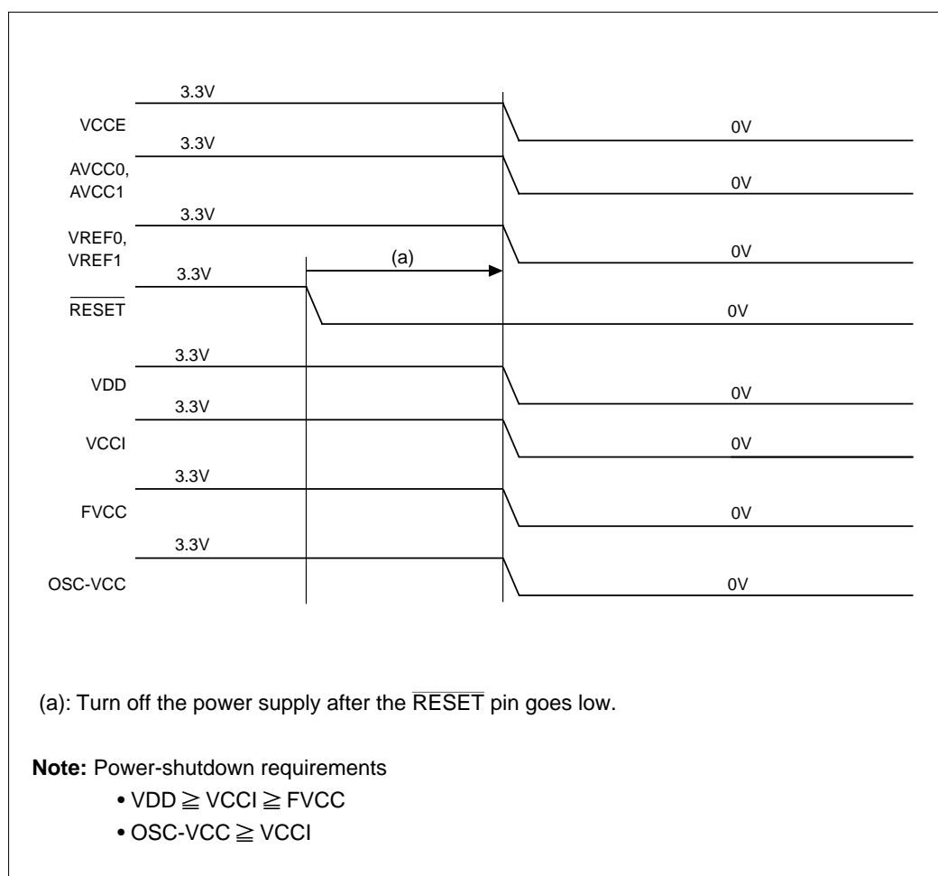
Figure 20.3.2 Power-Shutdown Sequence When Not Using RAM Backup (when VCC=3.3V)
