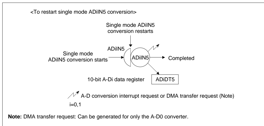
Figure 11.1.9 Restarting Conversion during Single Mode Operation
