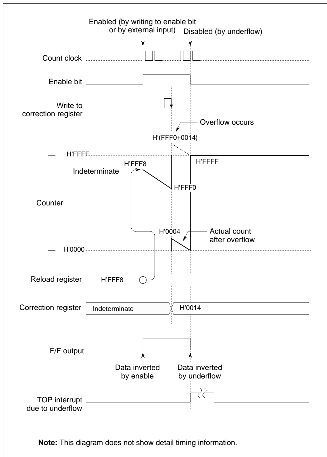
Figure 10.3.14 Example of Operation in TOP Single-shot Output Mode Where Count Overflows due to Correction
