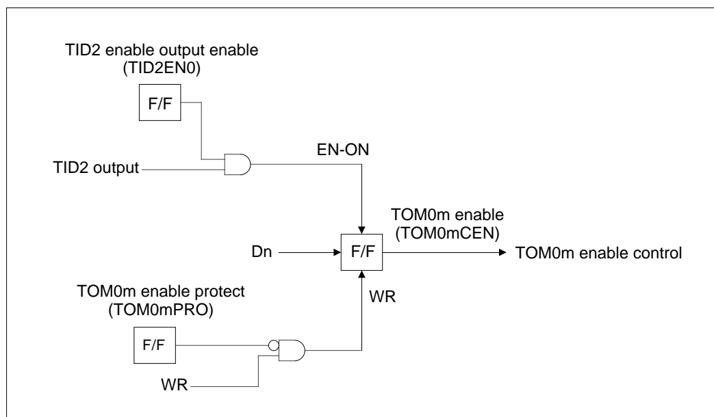
Figure 10.9.5 Configuration of the TOM Enable Circuit
