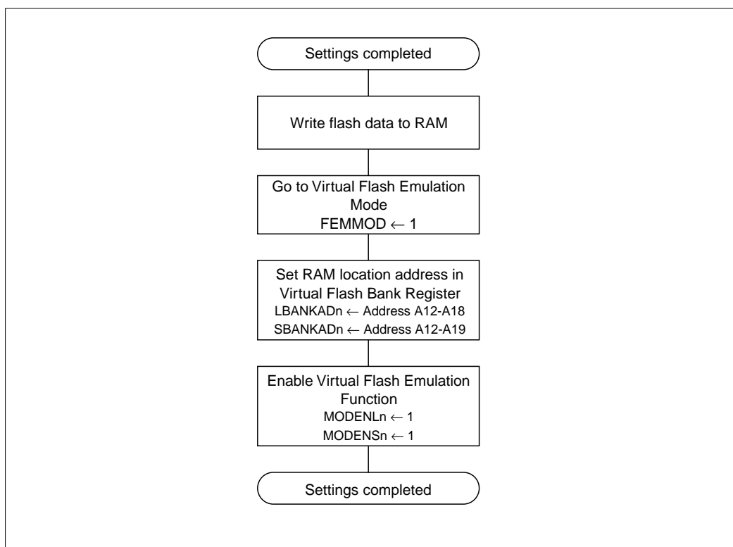
Figure 6.7.20 Virtual Flash Emulation Mode Sequence
