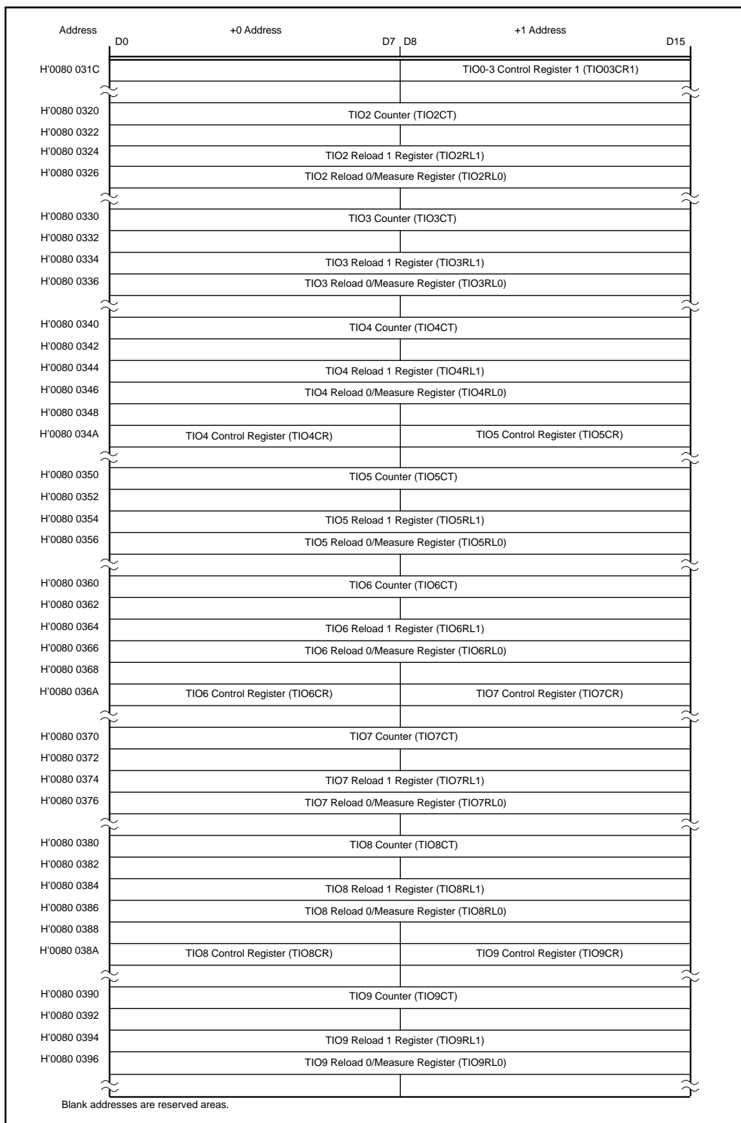
Figure 3.4.9 Register Mapping of the SFR Area (5)
