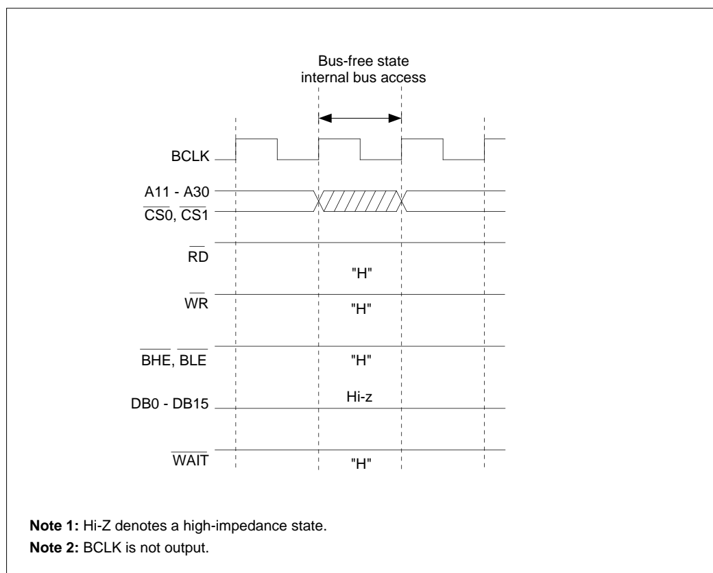
Figure 15.2.4 Internal Bus Access during Bus Free State
