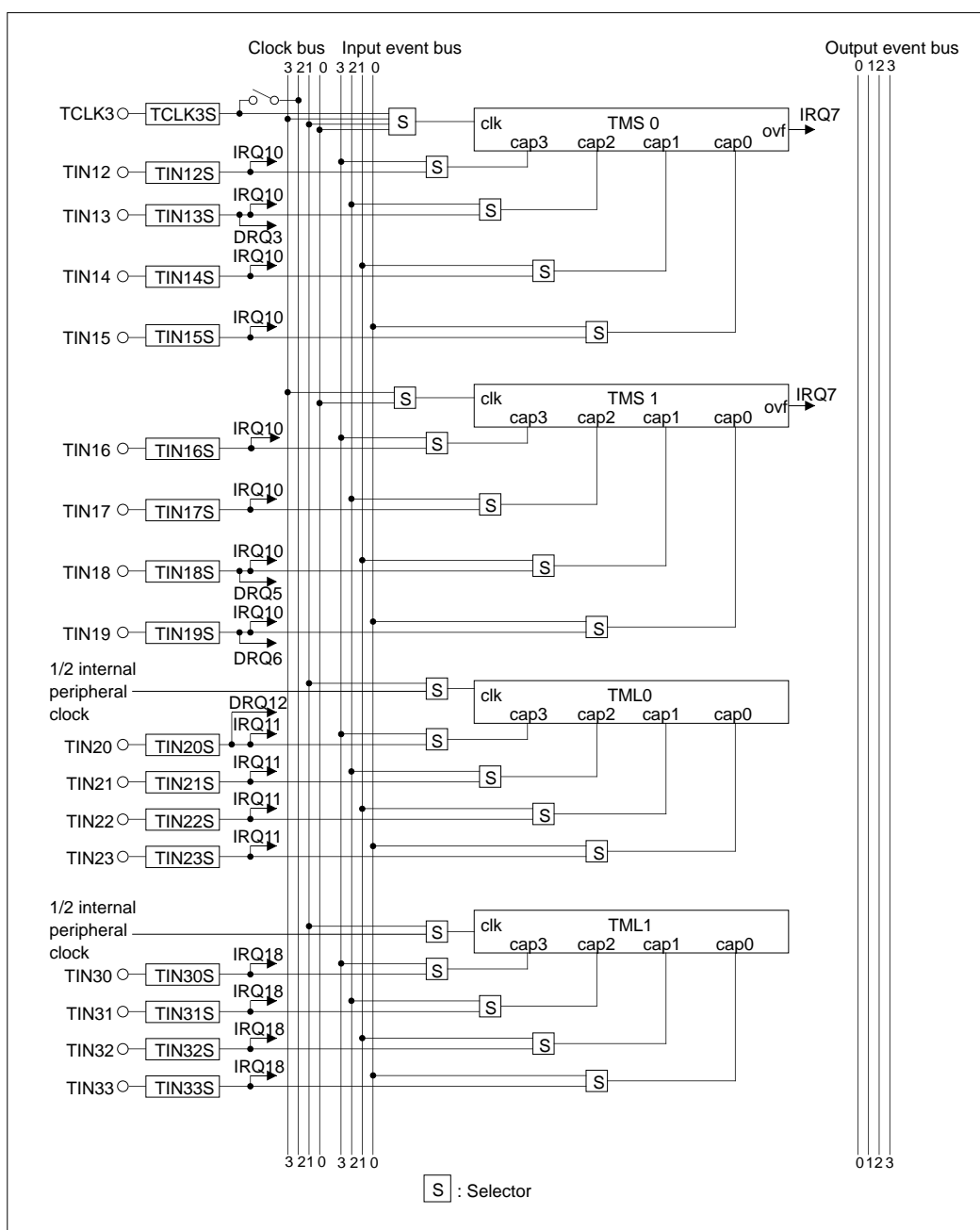
Figure 10.1.2 Block Diagram of MJT (2/4)
