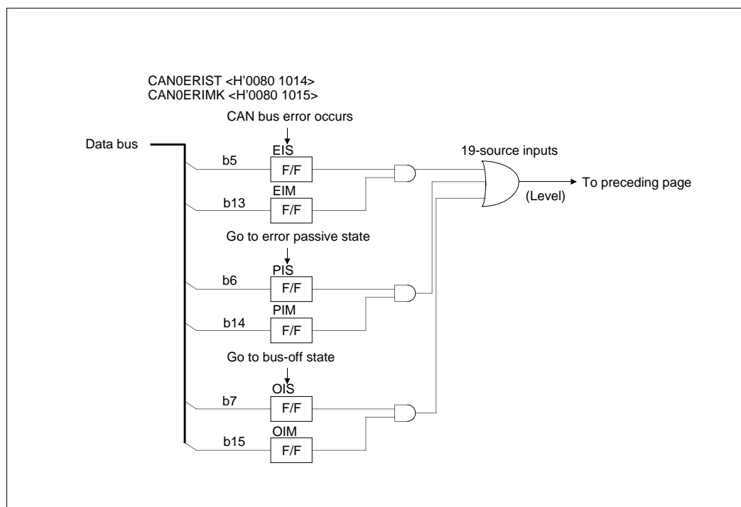
Figure 13.2.7 Block Diagram of CAN0 Group Interrupts (3/3)
