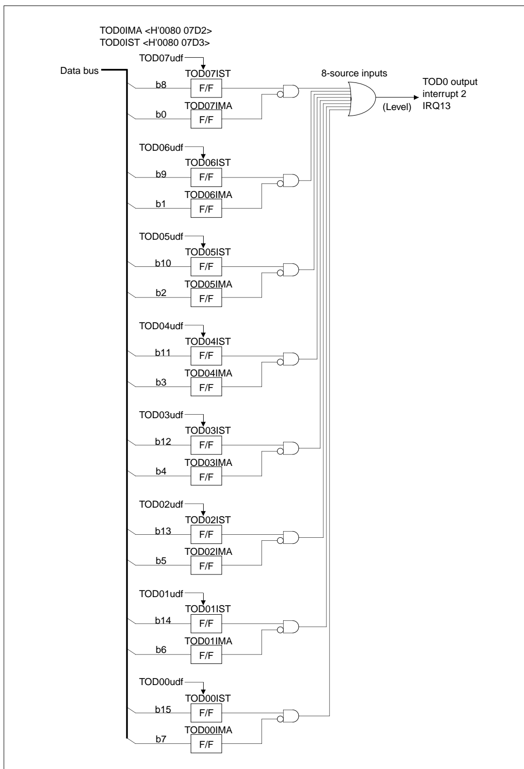
Figure 10.2.20 Block Diagram of TOD0 Output Interrupt
