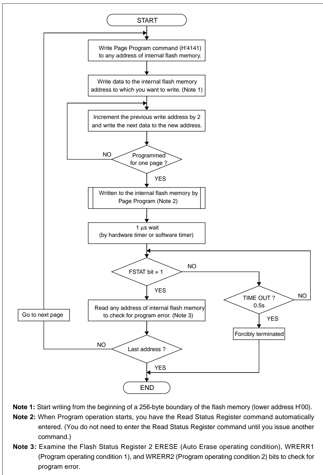
Figure 6.5.11 Page Program
