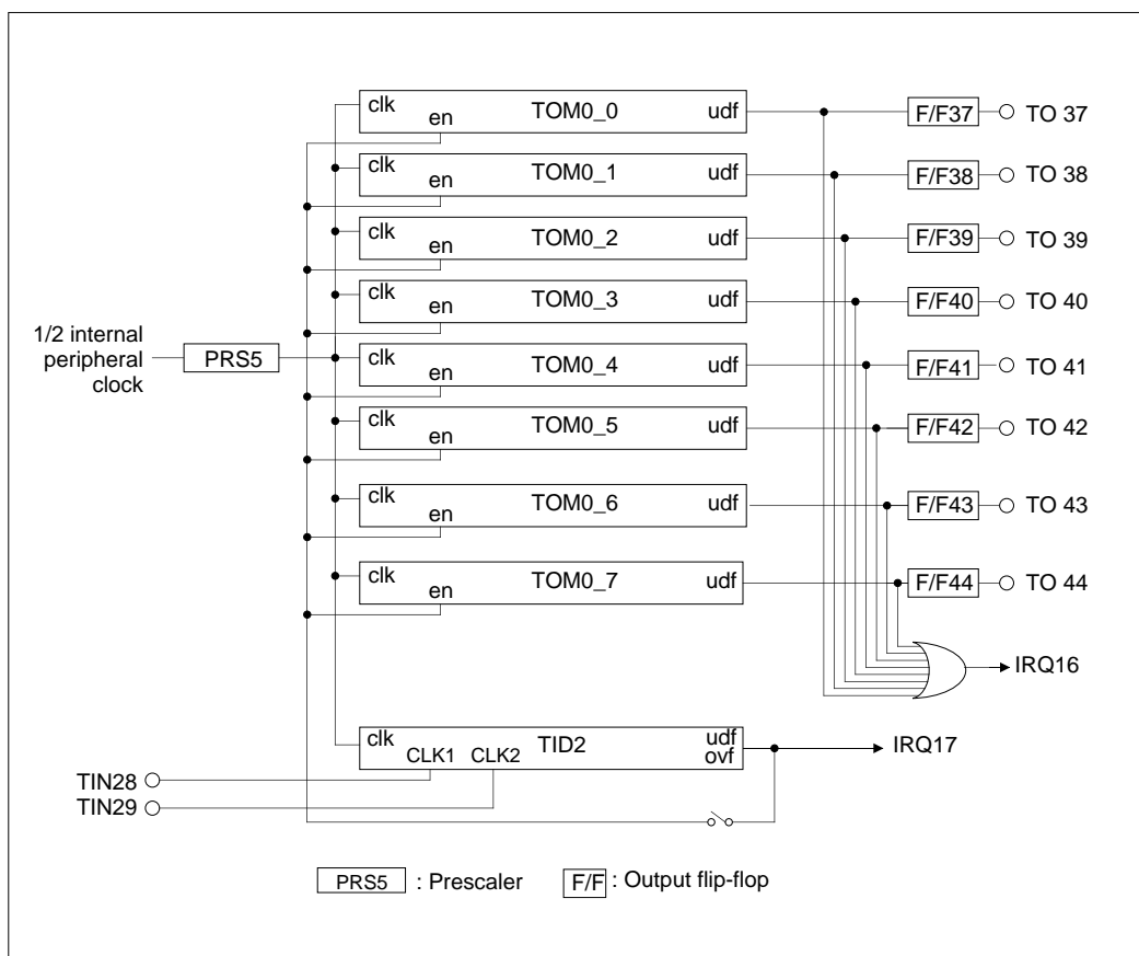
Figure 10.9.1 TOM (Output-related 16-bit Timer)
