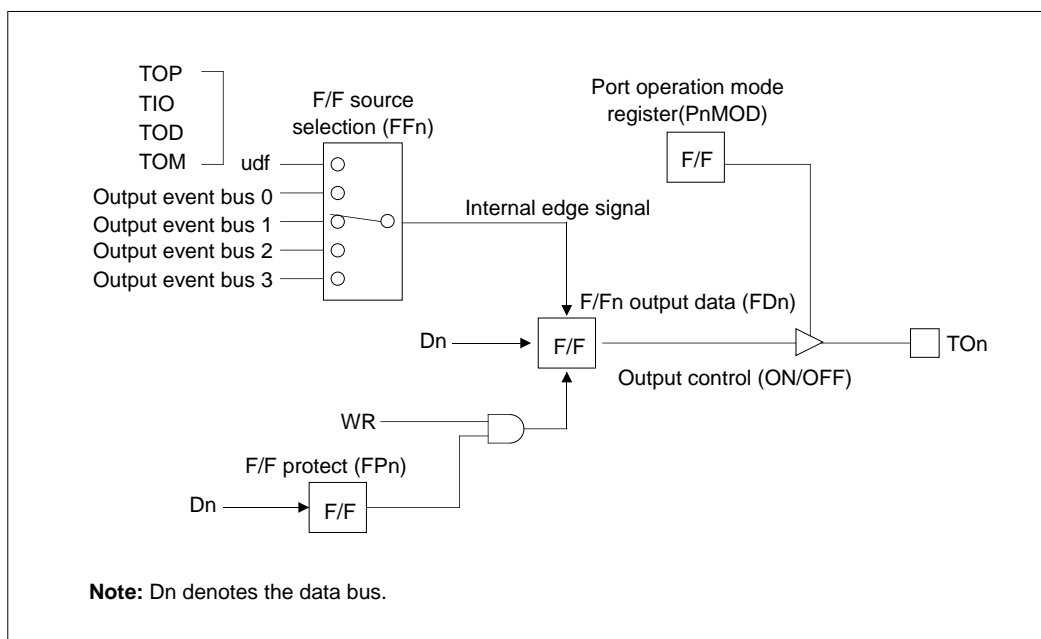
Figure 10.2.4 Configuration of the F/F Output Circuit
