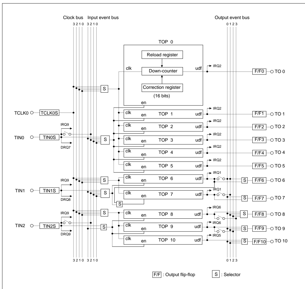
Figure 10.3.1 Block Diagram of TOP (Output-related 16-bit Timer)
