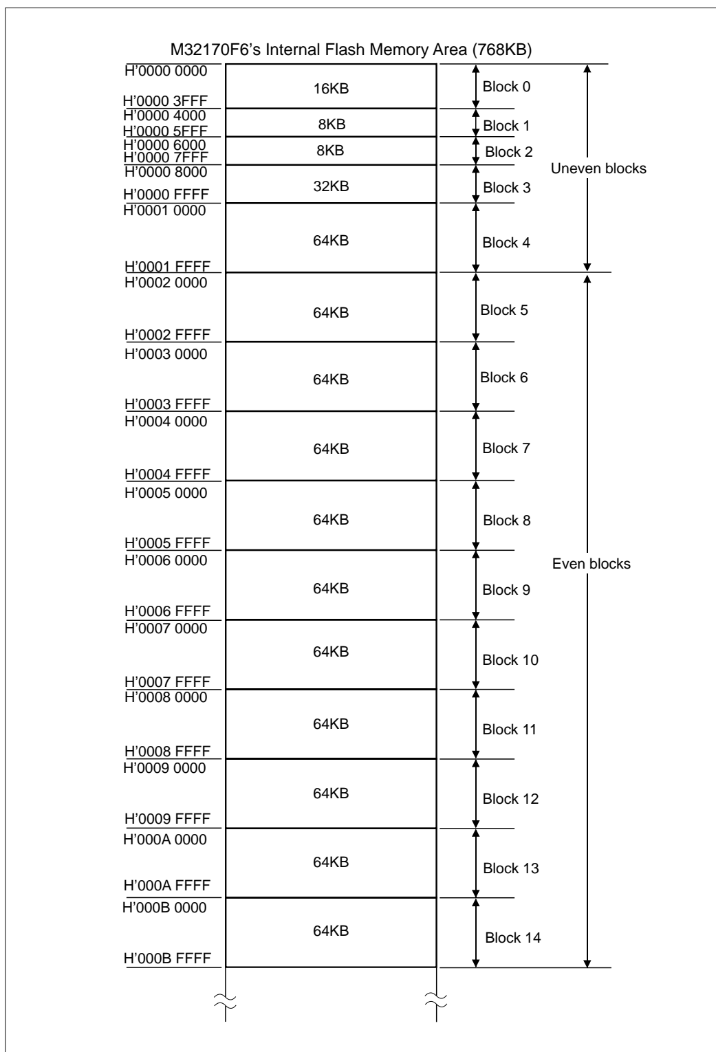
Figure 6.5.7 Block Configuration of the M32170F6 Flash Memory
