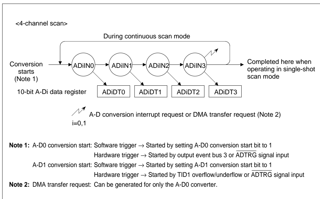
Figure 11.1.5 Operation of A-D Conversion in Scan Mode (for 4-channel Scan)
