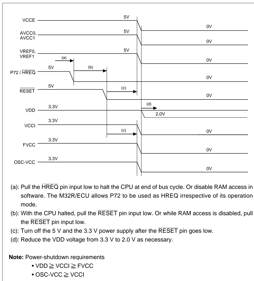
Figure 20.3.3 Power-Shutdown Sequence When Using RAM Backup(when VCC=5V)
