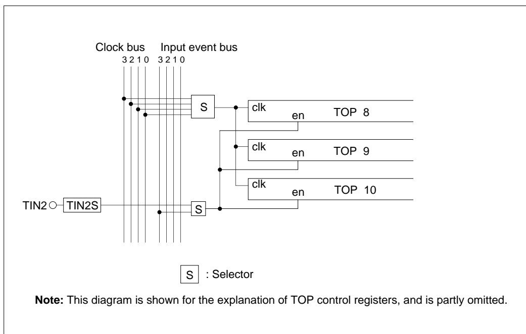
Figure 10.3.7 Outline Diagram of TOP8-10 Clock/Enable Inputs
