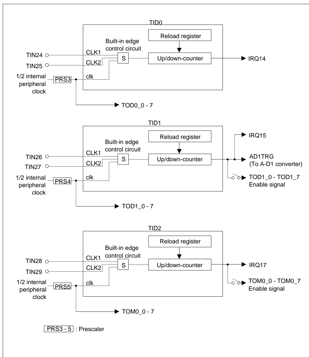
Figure 10.7.1 Block Diagram of TID (Input-related 16-bit Timer)
