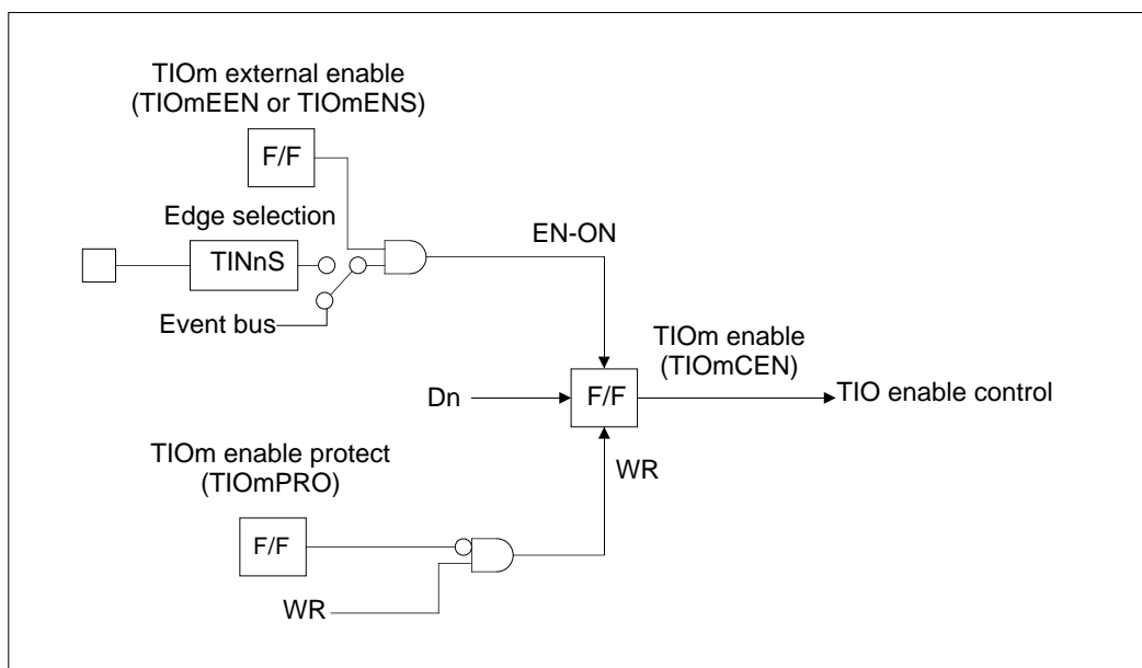
Figure 10.4.7 Configuration of the TIO Enable Circuit
