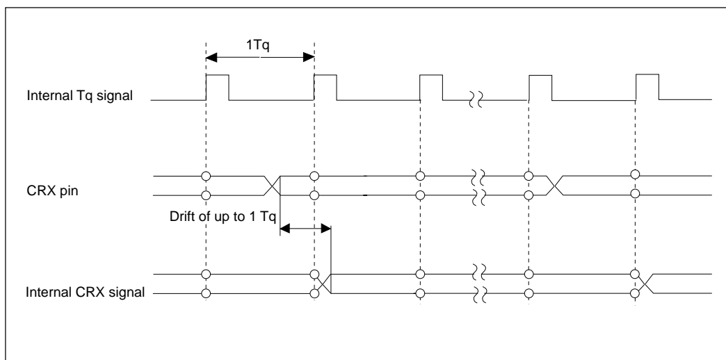
Figure 13.4.3 Operation Timing
