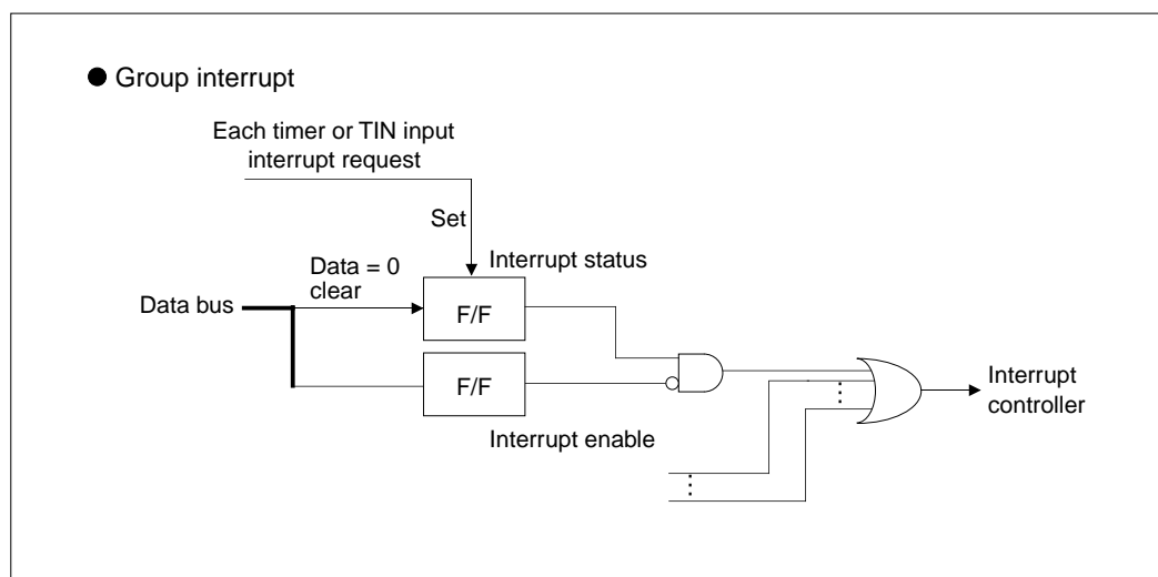
Figure 10.2.5 Interrupt Status Register and Mask Register
