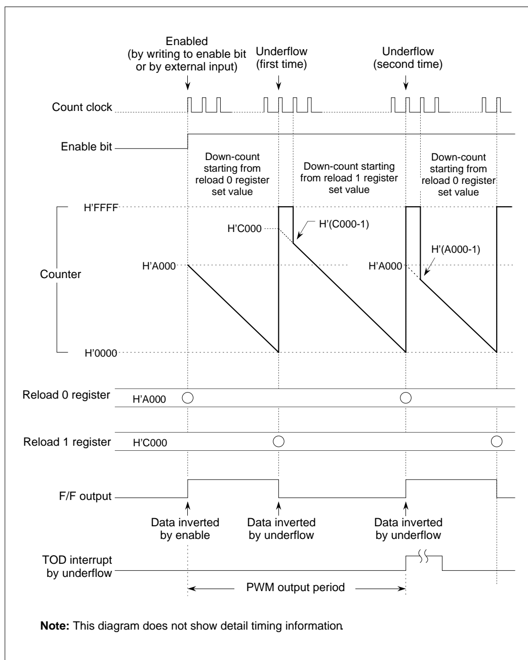
Figure 10.8.8 Typical Operation in PWM Output Mode
