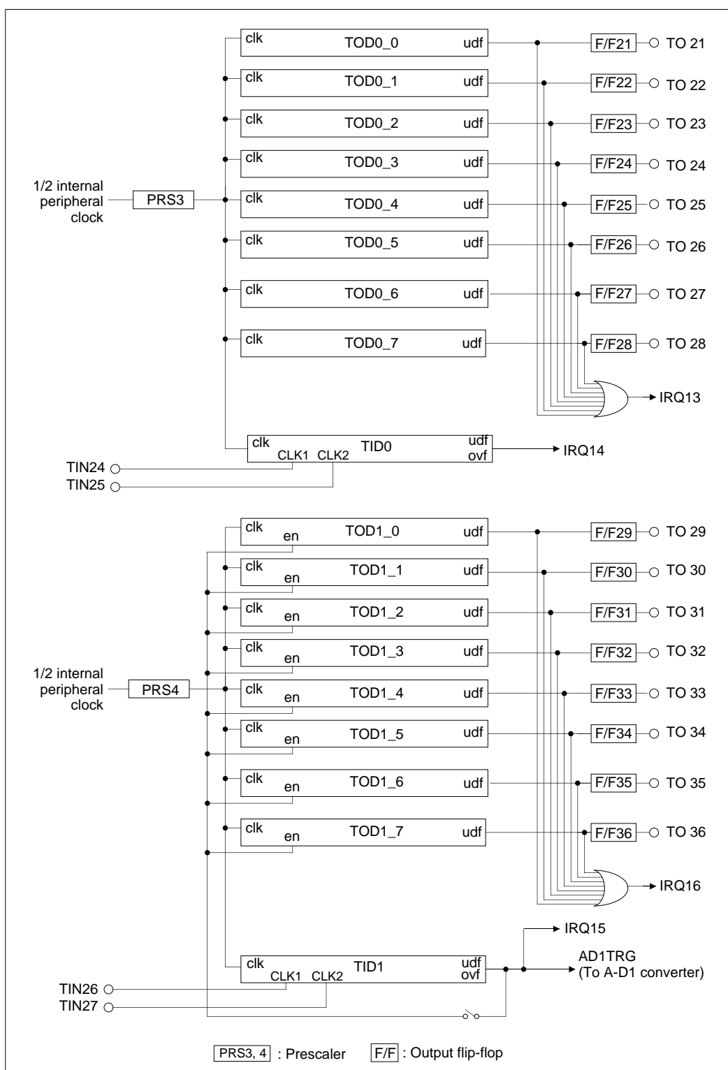
Figure 10.8.1 Block Diagram of TOD (Output-related 16-bit Timer)
