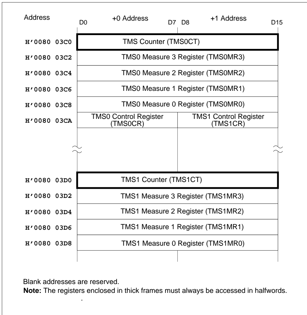
Figure 10.5.2 TMS Related Register Map
