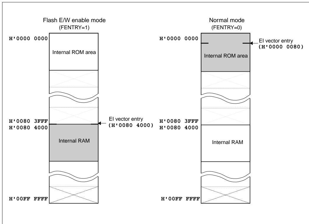
Figure 6.5.1 El Vector Entry When in Flash E/W Enable Mode
