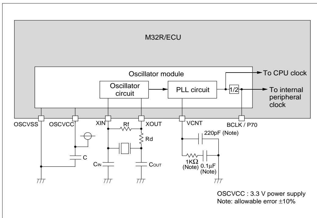
Figure 18.1.1 Example of a System Clock Generating Circuit
