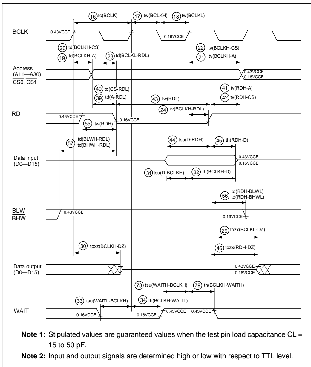
Figure 21.3.6 Read Timing
