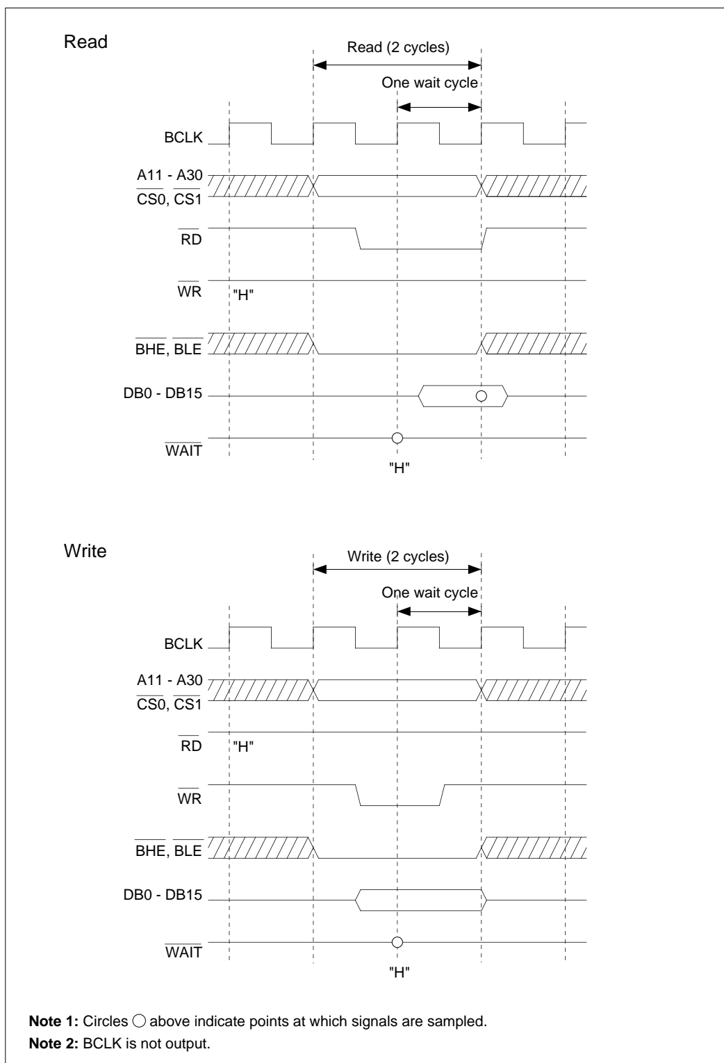
Figure 15.2.5 Read/Write Timing (for Shortest-case External Access)
