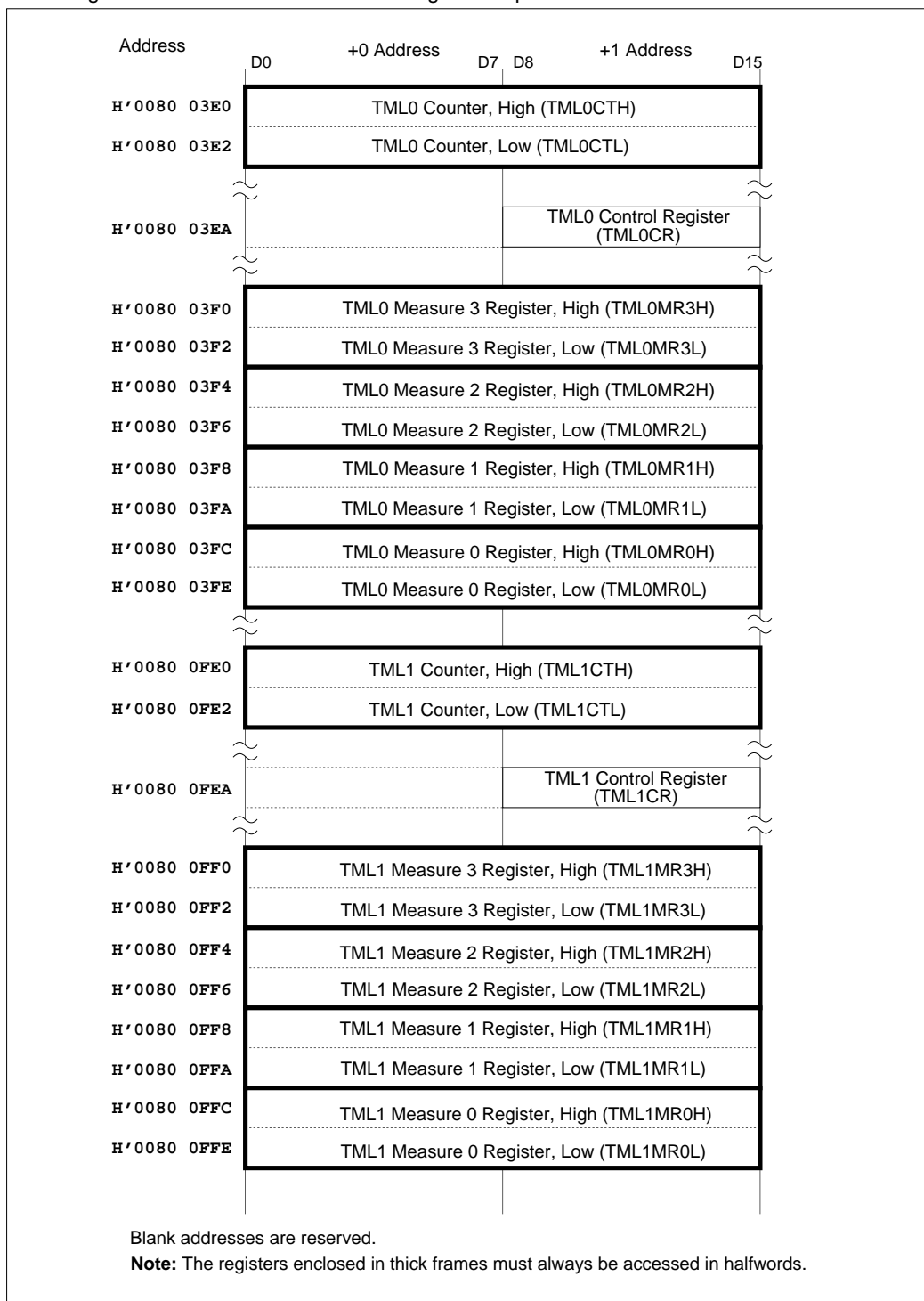
Figure 10.6.2 TML Related Register Map
