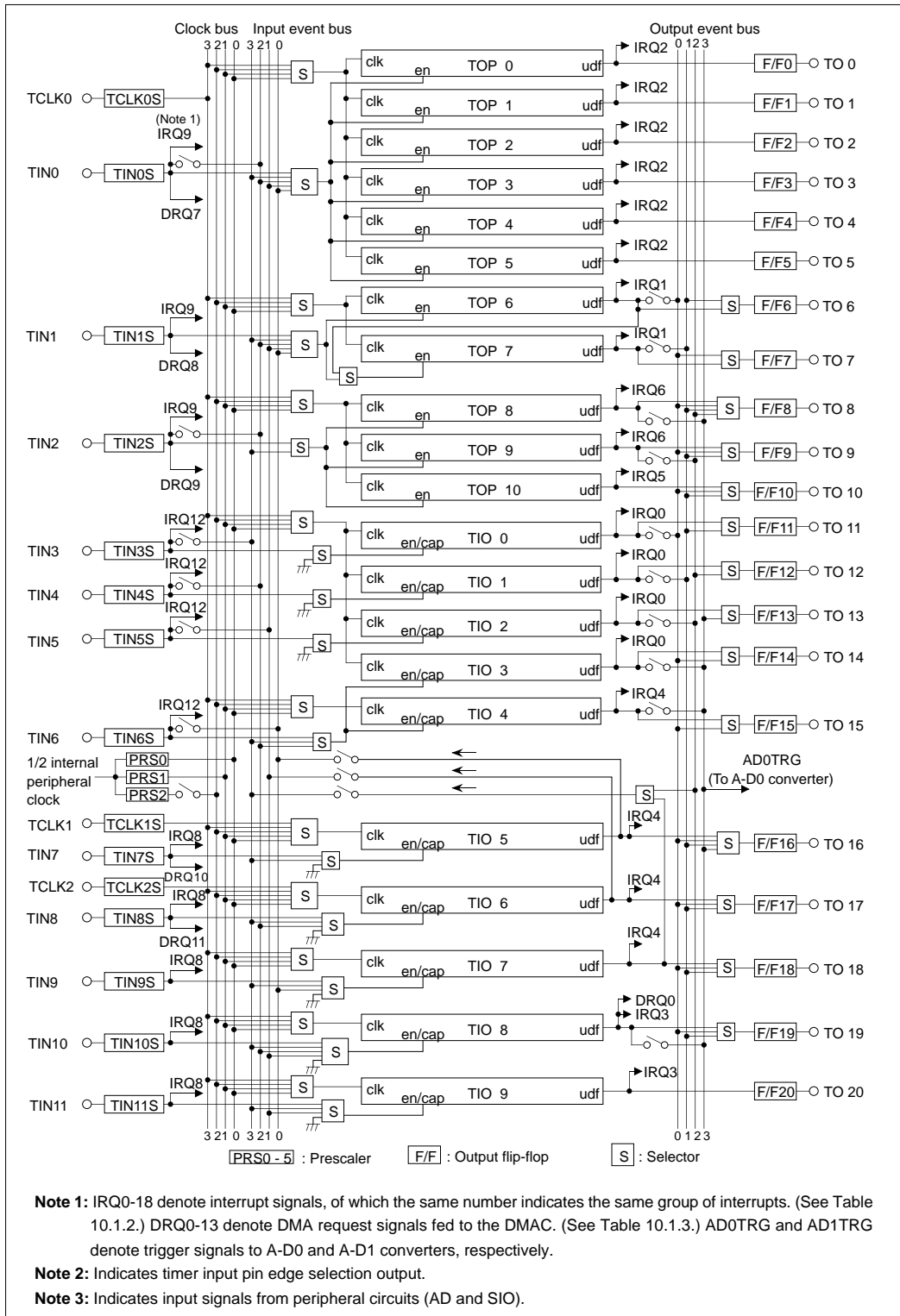
Figure 10.1.1 Block Diagram of MJT (1/4)
