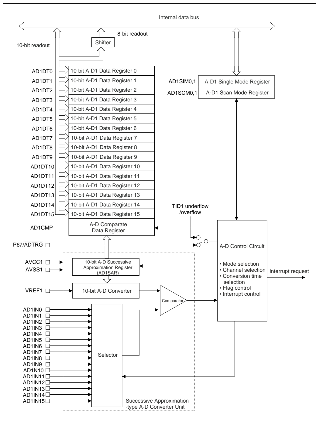
Figure 11.1.2 Block Diagram of A-D0 Converter
