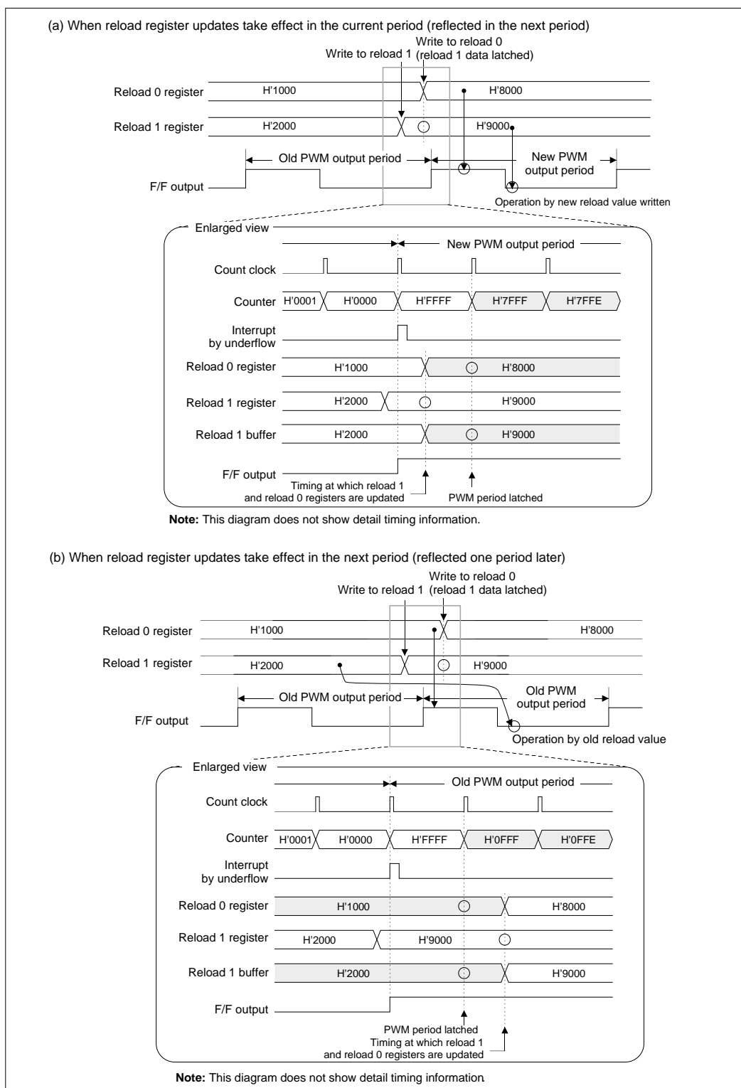
Figure 10.8.10 Reload 0 and Reload 1 Register Updates in PWM Output Mode
