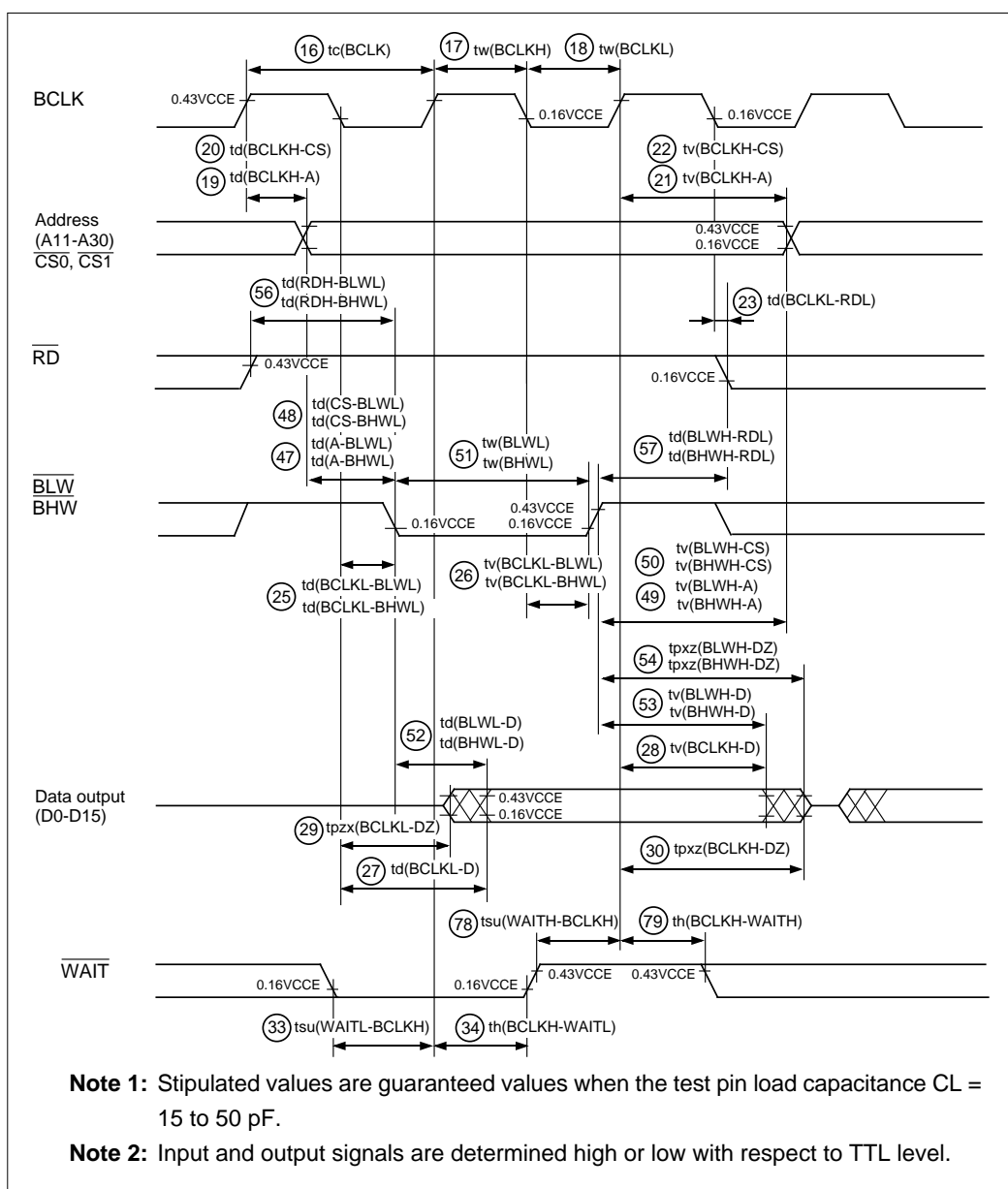
Figure 21.3.7 Write Timing
