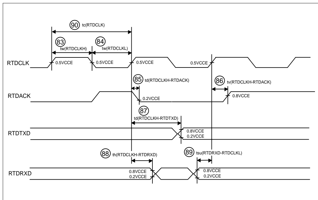
Figure 21.3.12 RTD Timing
