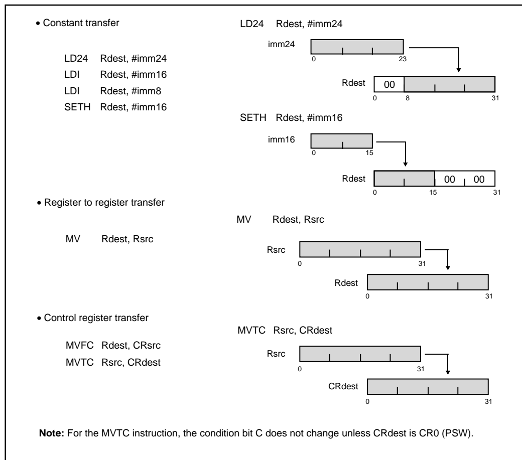
Figure 2.6.6 Transfer instructions
