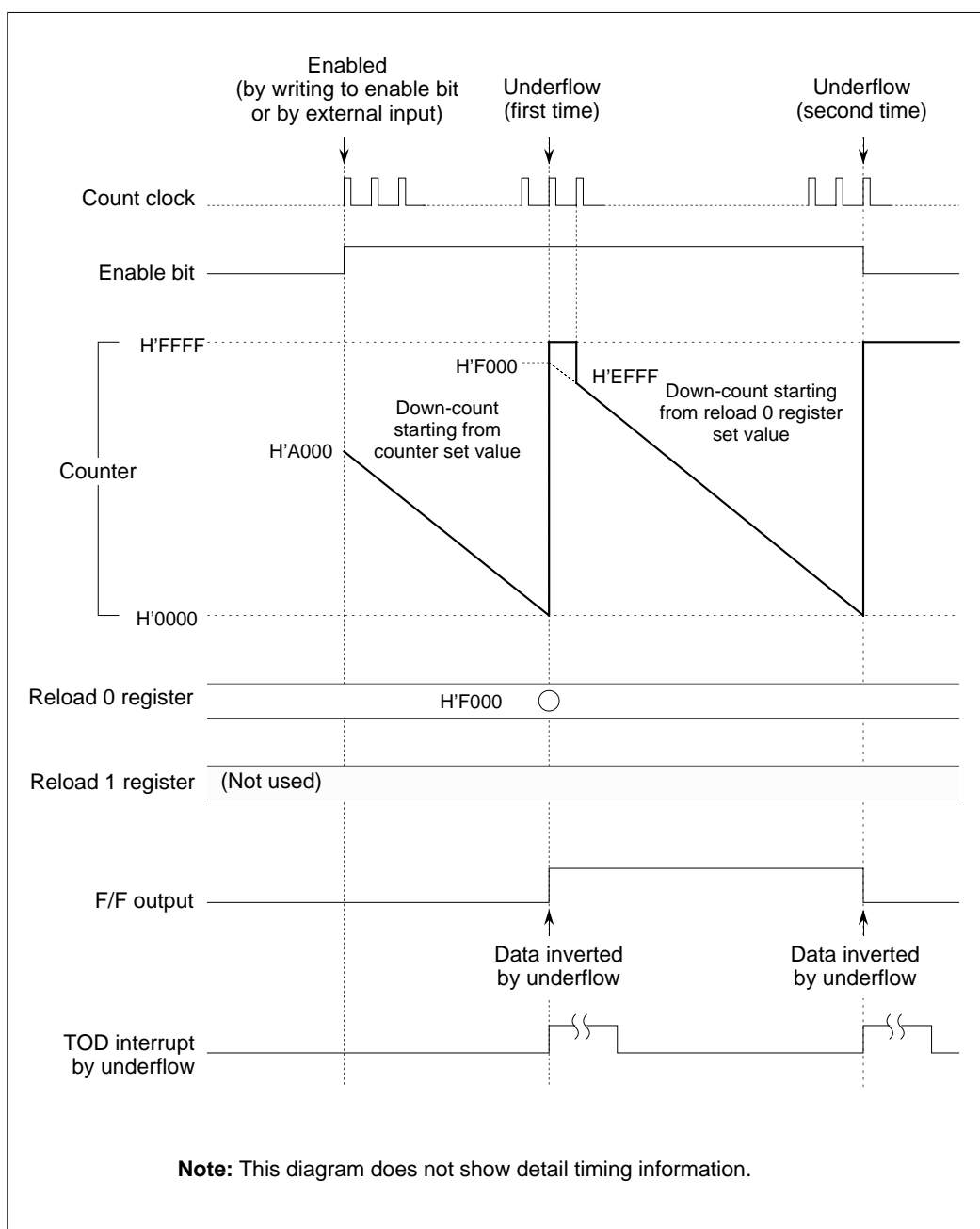
Figure 10.8.12 Typical Operation in TOD Delayed Single-shot Output Mode (without Correction Function)
