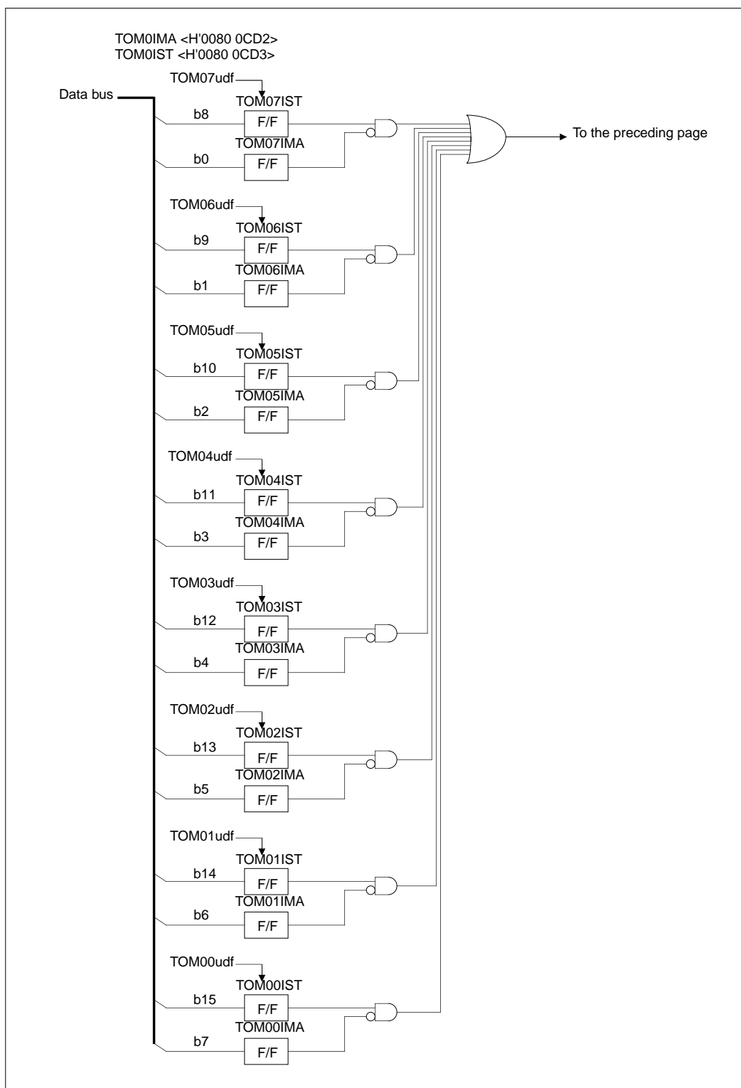
Figure 10.2.22 Block Diagram of TOD1 + TOM0 Output Interrupt (2/2)
