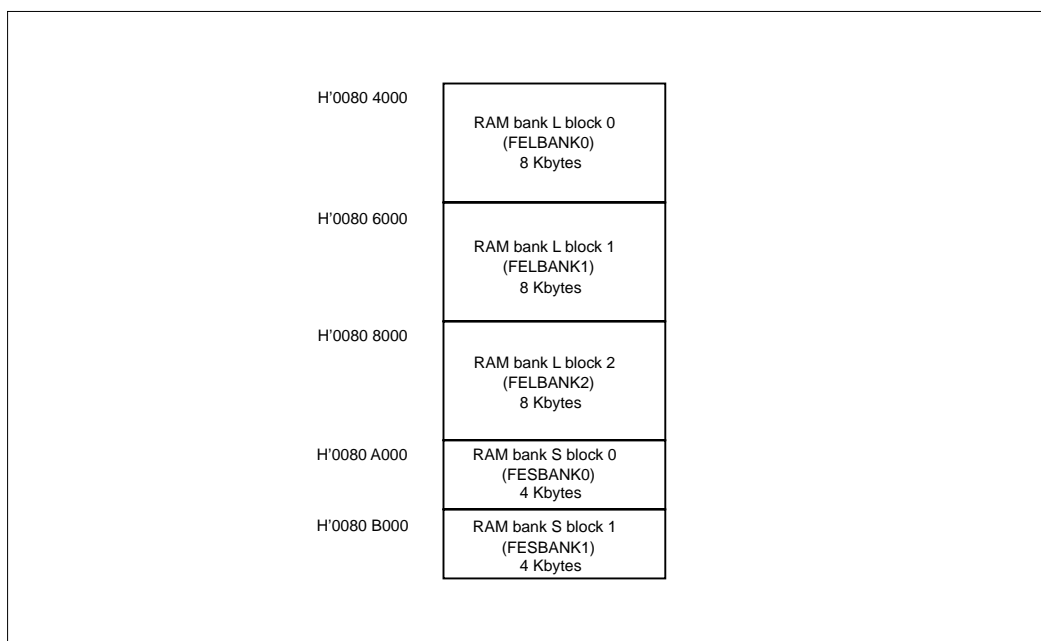
Figure 6.7.2 Internal RAM Bank Configuration of the M32170F4 and M32170F3
