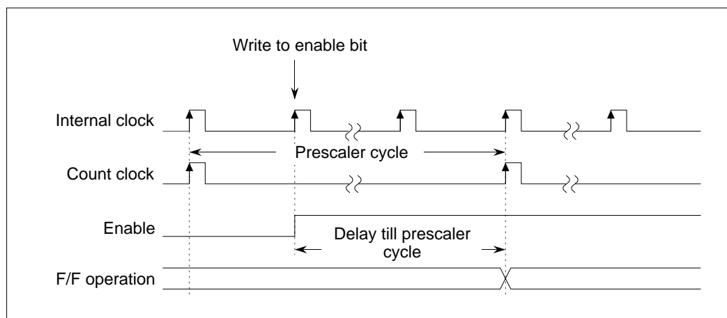
Figure 10.3.13 Prescaler Delay
