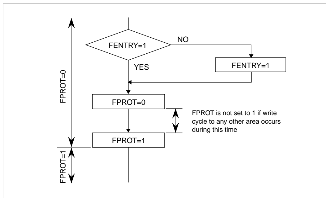
Figure 6.4.2 Protection Unlocking Flow
