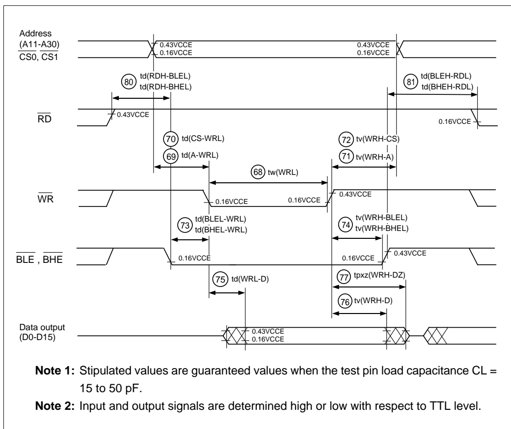
Figure 21.3.8 Write Timing (Byte enable mode)
