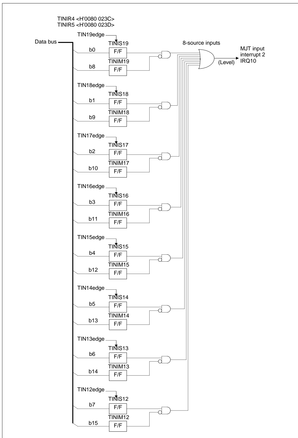
Figure 10.2.17 Block Diagram of MJT Input Interrupt 2
