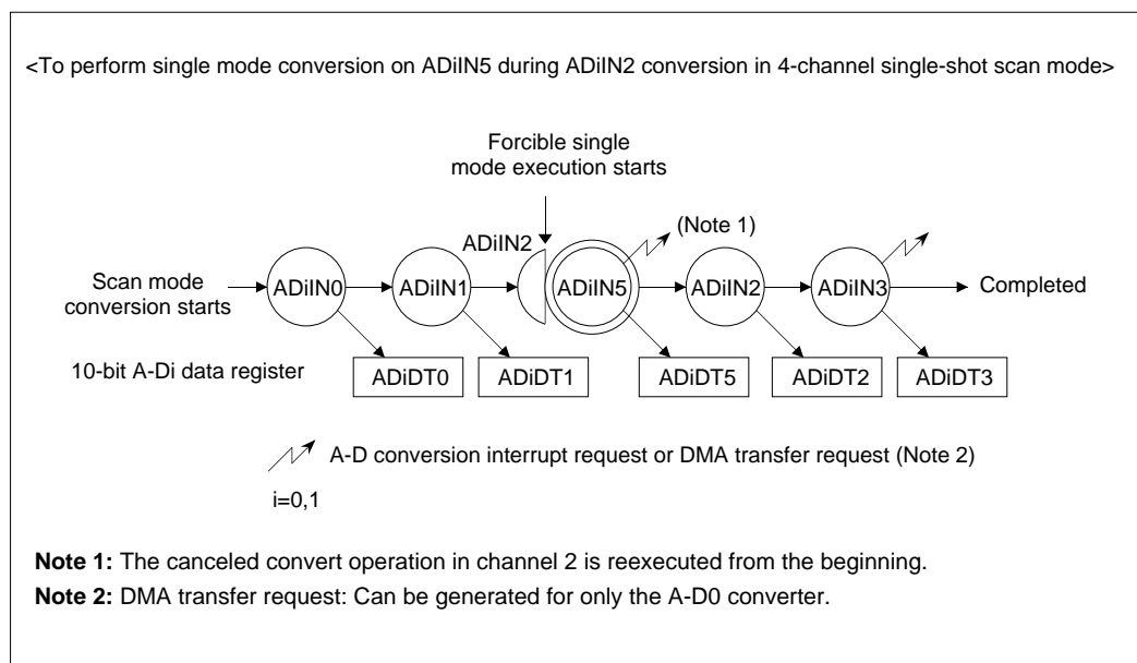
Figure 11.1.7 Forcible Single Mode Execution during Scan Mode
