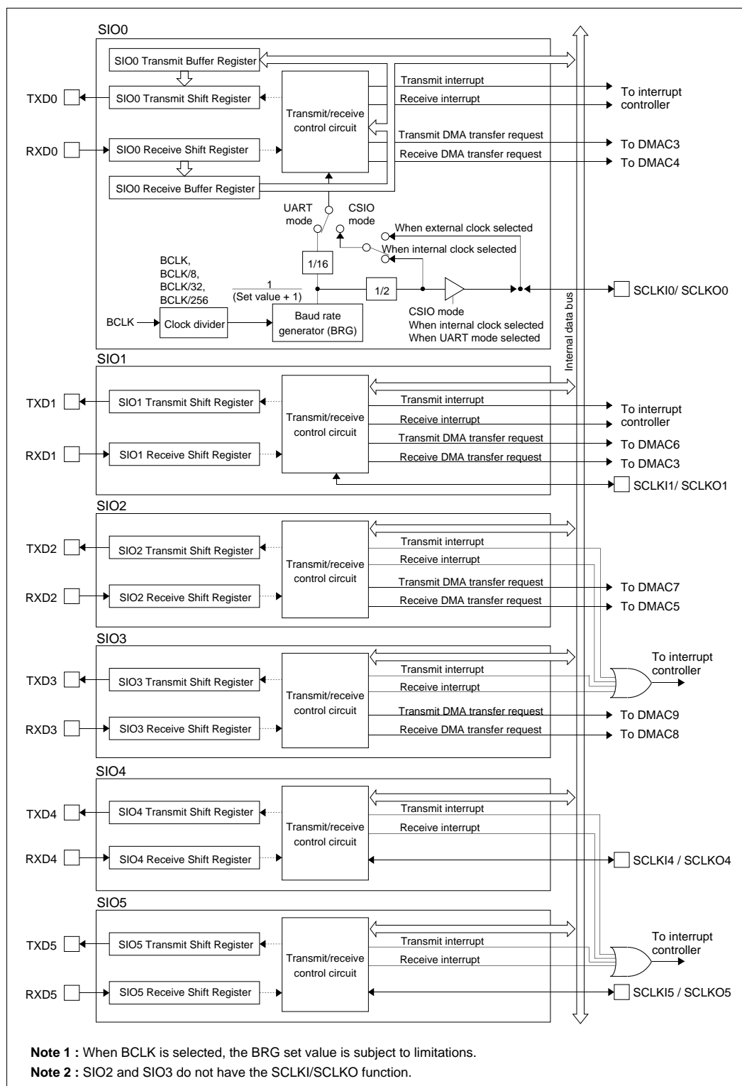
Figure 12.1.1 Block Diagram of SIO0-SIO5
