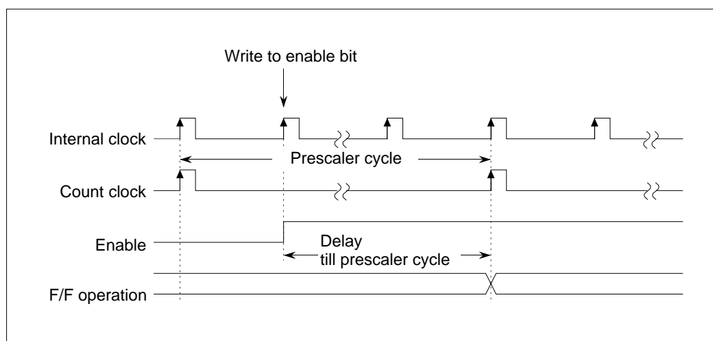
Figure 10.3.22 Prescaler Delay
