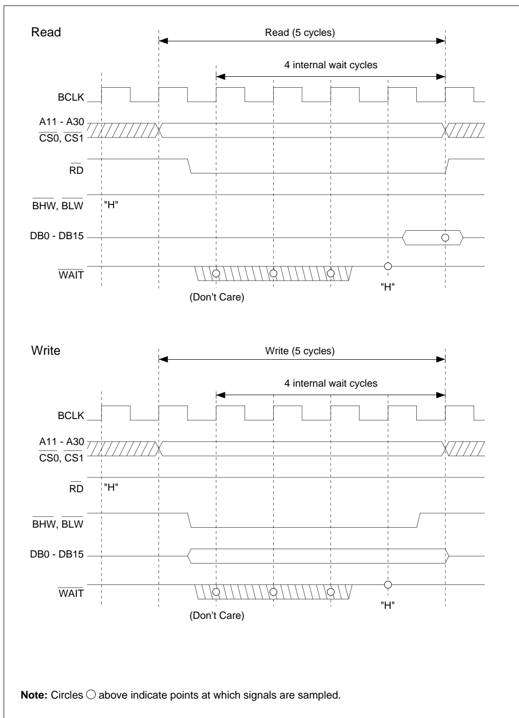
Figure 16.3.5 Read/Write Timing (for Access with 4 Internal Wait Cycles)
