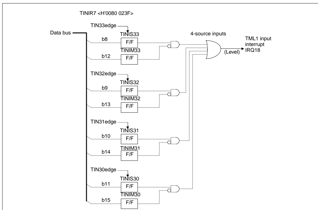
Figure 10.2.19 Block Diagram of TML1 Input Interrupt
