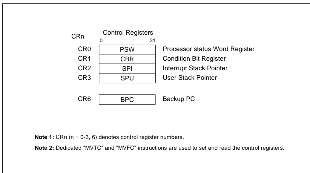
Figure 2.3.1 Control Registers
