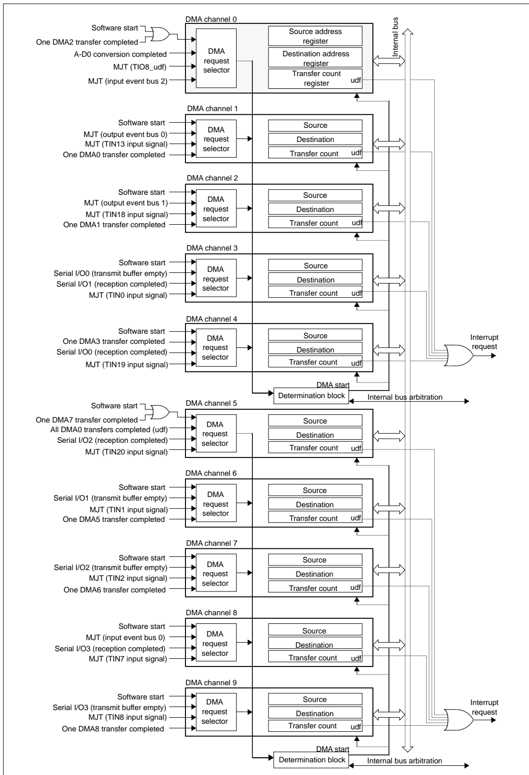
Figure 9.1.1 Block Diagram of the DMAC
