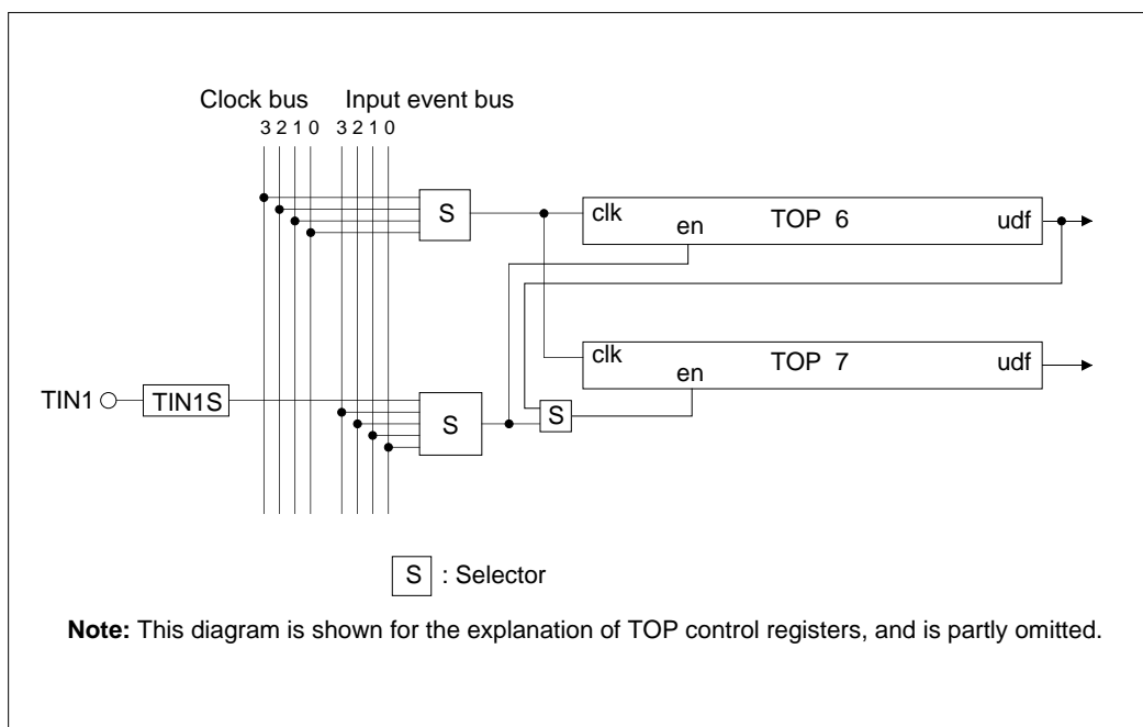
Figure 10.3.6 Outline Diagram of TOP6, TOP7 Clock/Enable Inputs
