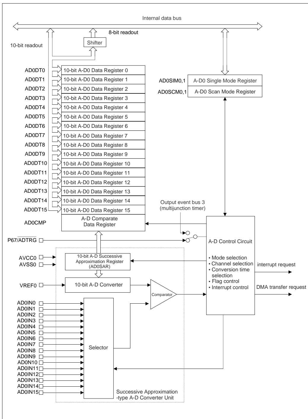
Figure 11.1.1 Block Diagram of A-D0 Converter
