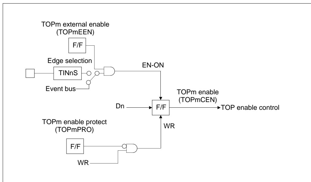
Figure 10.3.8 Configuration of the TOP Enable Circuit
