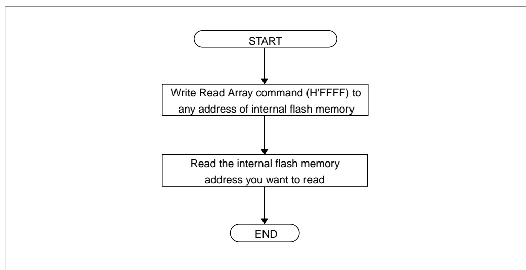
Figure 6.5.10 Read Array
