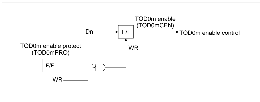
Figure 10.8.6 Configuration of TOD0 Enable Circuit
