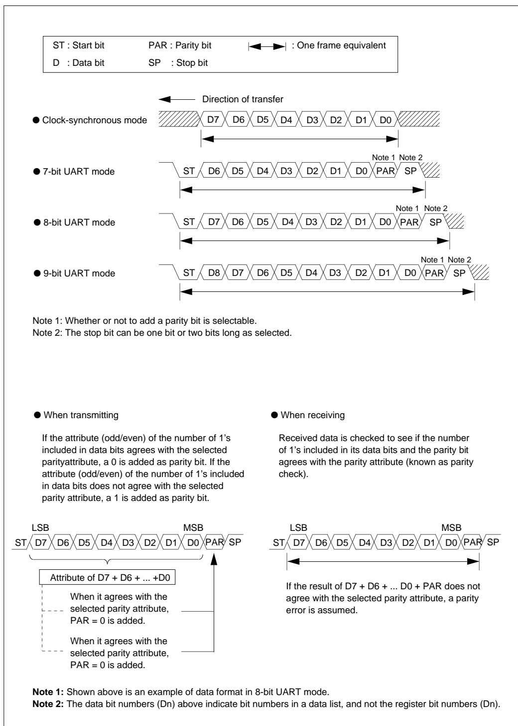
Figure 12.2.4 Data Format when Parity is Enabled
