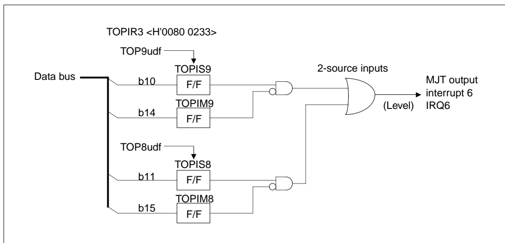
Figure 10.2.9 Block Diagram of MJT Output Interrupt 6
