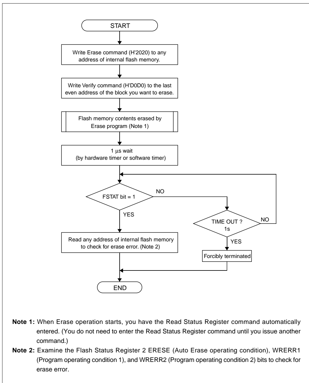
Figure 6.5.13 Block Erase
