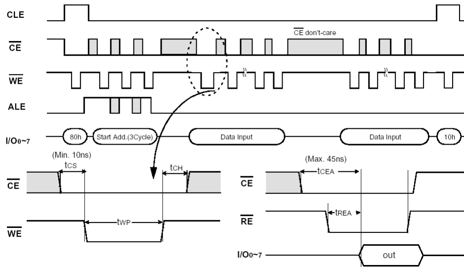
FIGURE 8. PROGRAM OPERATION WITH \overline{\text{CE}} DON'T CARE
