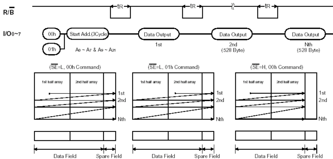
FIGURE 25. SEQUENTIAL READ2 OPERATION ( \overline{SE} = FIXED LOW)
