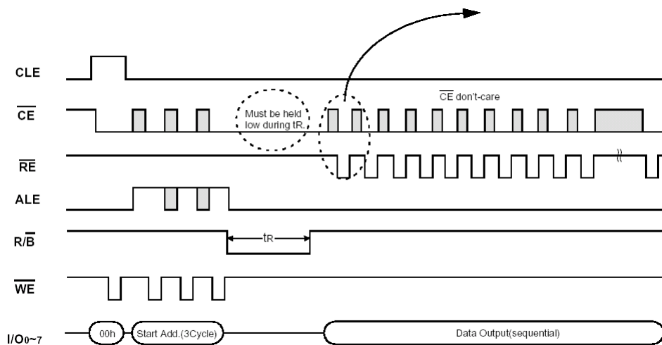
FIGURE 9. READ OPERATION WITH \overline{\text{CE}} DON'T CARE
