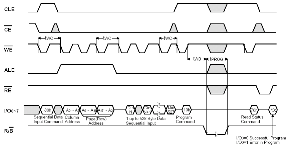
FIGURE 19. PAGE PROGRAM OPERATION
