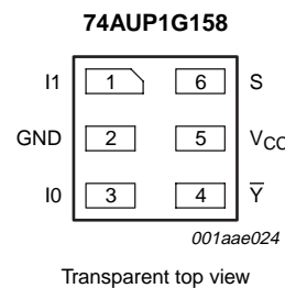
Fig 7. Pin configuration SOT891 (XSON6)
