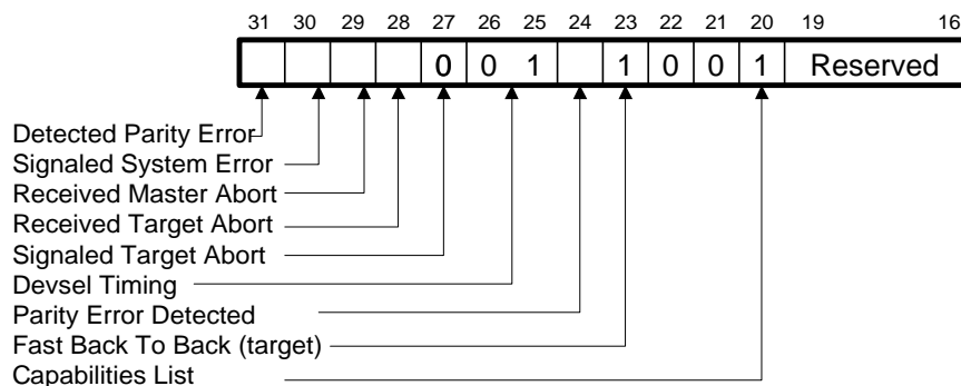
Figure 15. PCI Status Register
